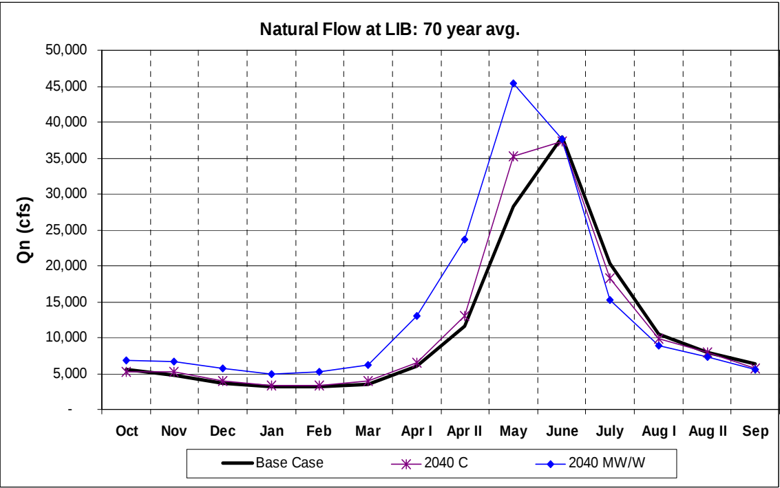
Figure 144. Libby Natural Inflows for 2040s.
