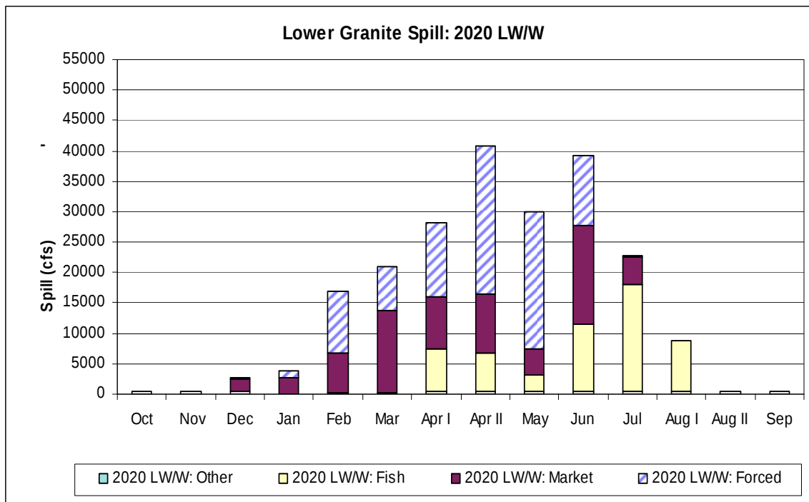
Figure 153. 2020 LW/W Scenario: Lower Granite Spill Breakdown.
