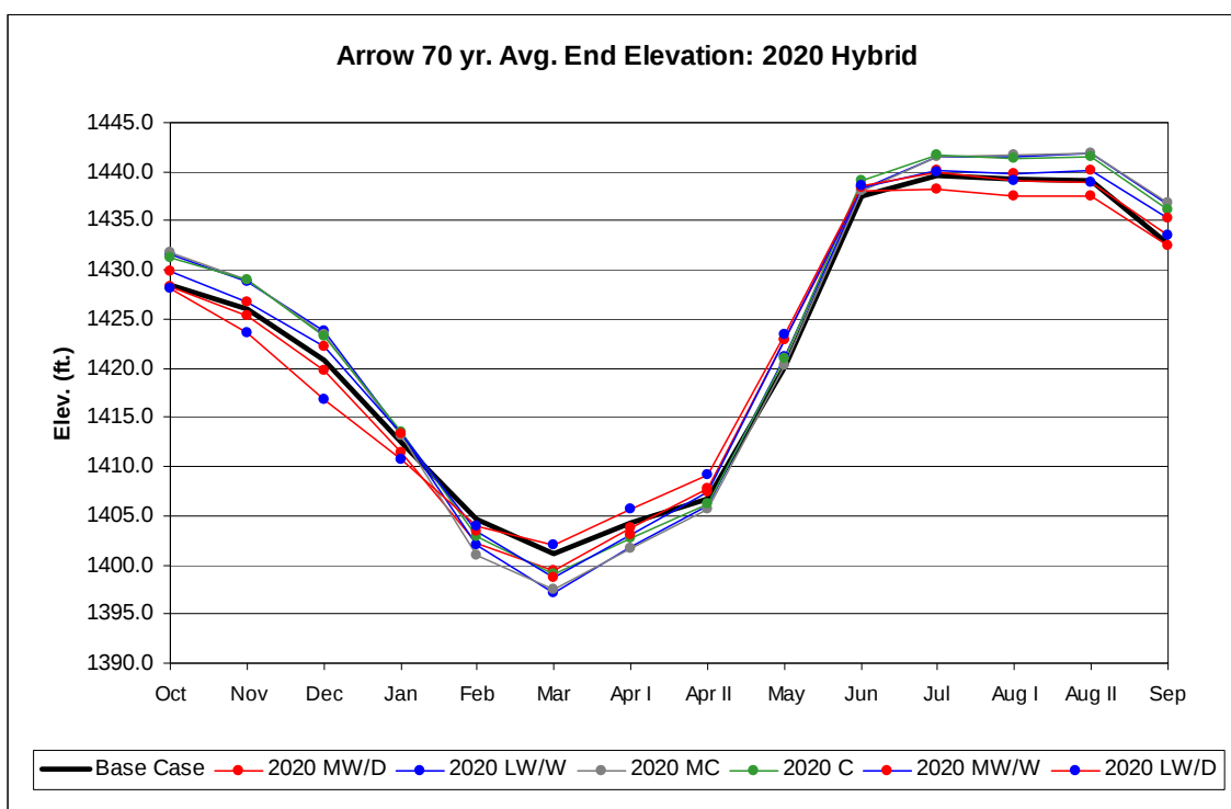
Figure 77. Arrow End Elevations: 2020s Hybrid-Delta.
