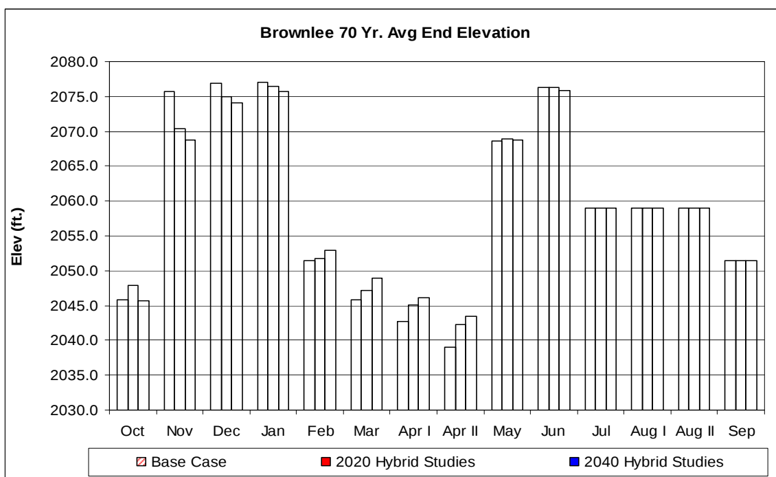
Figure 113. Comparison of period ending Brownlee reservoir elevation for the Base Case, 2020 Hybrid-Delta, and 2040 Hybrid-Delta climate change scenarios.
