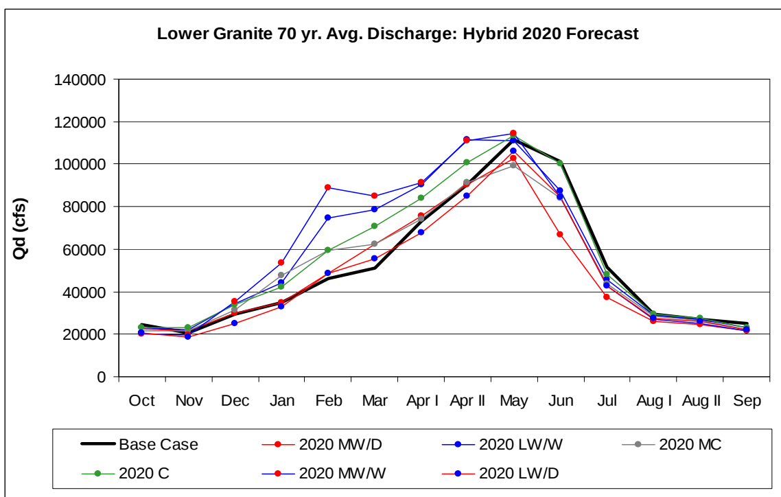
Figure 121. Lower Granite Discharge: 2020s Hybrid-Delta.
