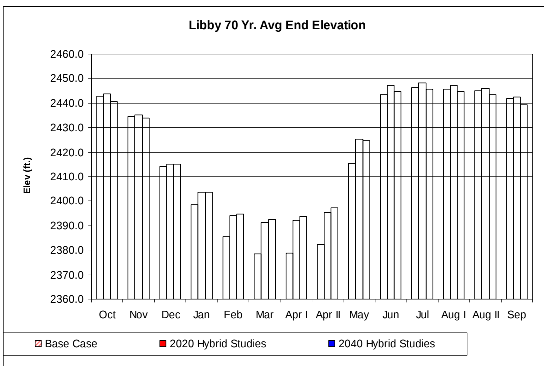
Figure 80. Libby Average End Elevation for Base Case and Climate Change Scenarios.
