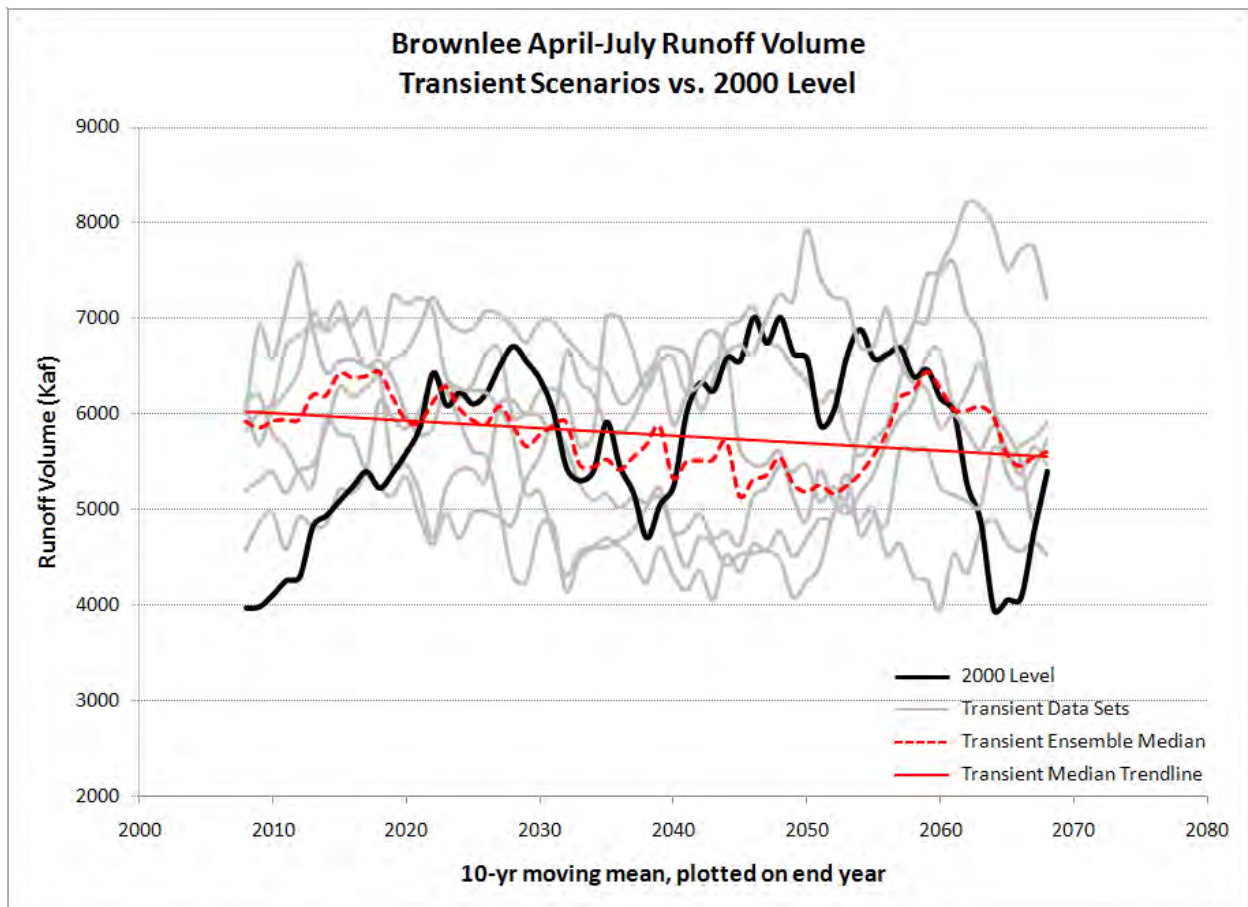
Figure 41. Brownlee Apr-Jul Runoff Volume Rolling Average – Transient.
