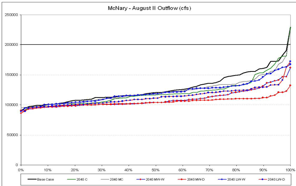
Figure 136. Comparison of 2040 Hybrid-Delta scenarios - August II McNary Outflow distributions.
