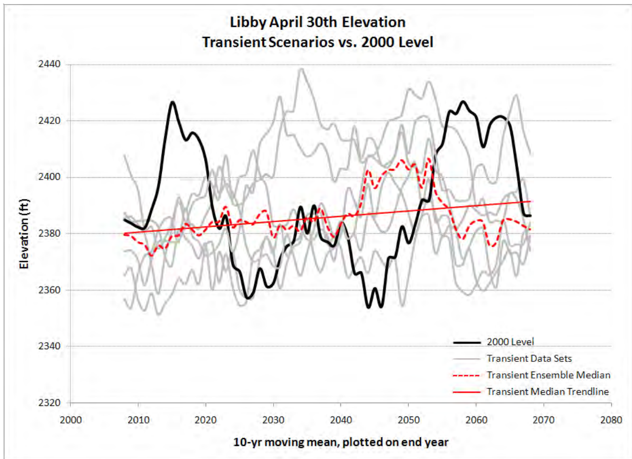
Figure 52. Libby April 30 Elevations Rolling Average – Transient.
