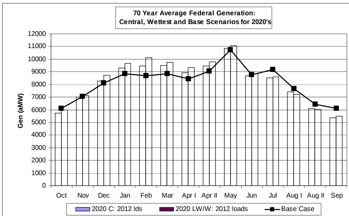
Figure 157. Federal Generation Comparison for Hybrid-Delat 2020s.
