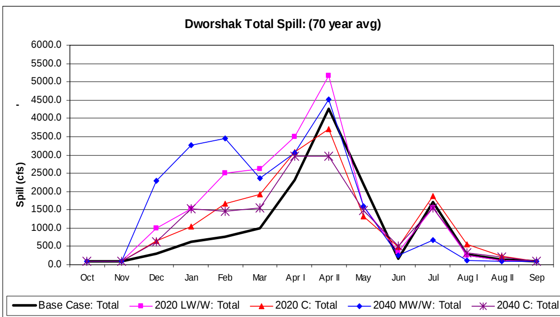
Figure 148. Dworshak Spill Comparison.
