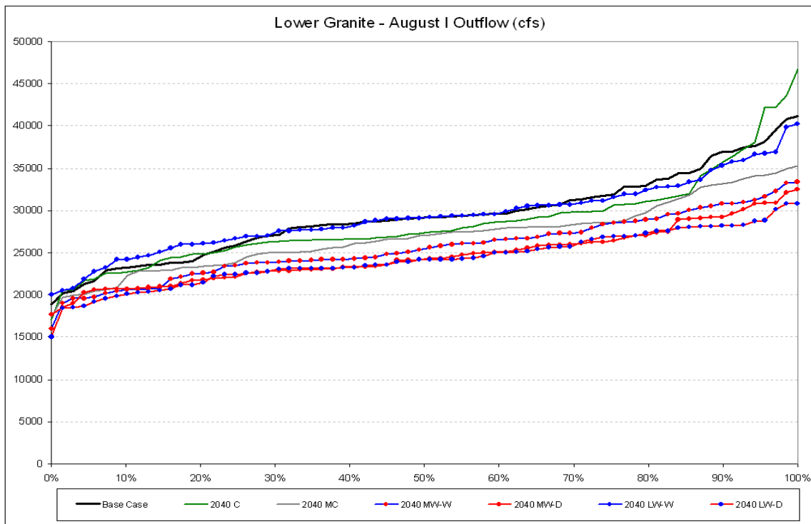
Figure 141. Comparison of 2040 Hybrid-Delta scenarios - August I Lower Granite outflow distributions.
