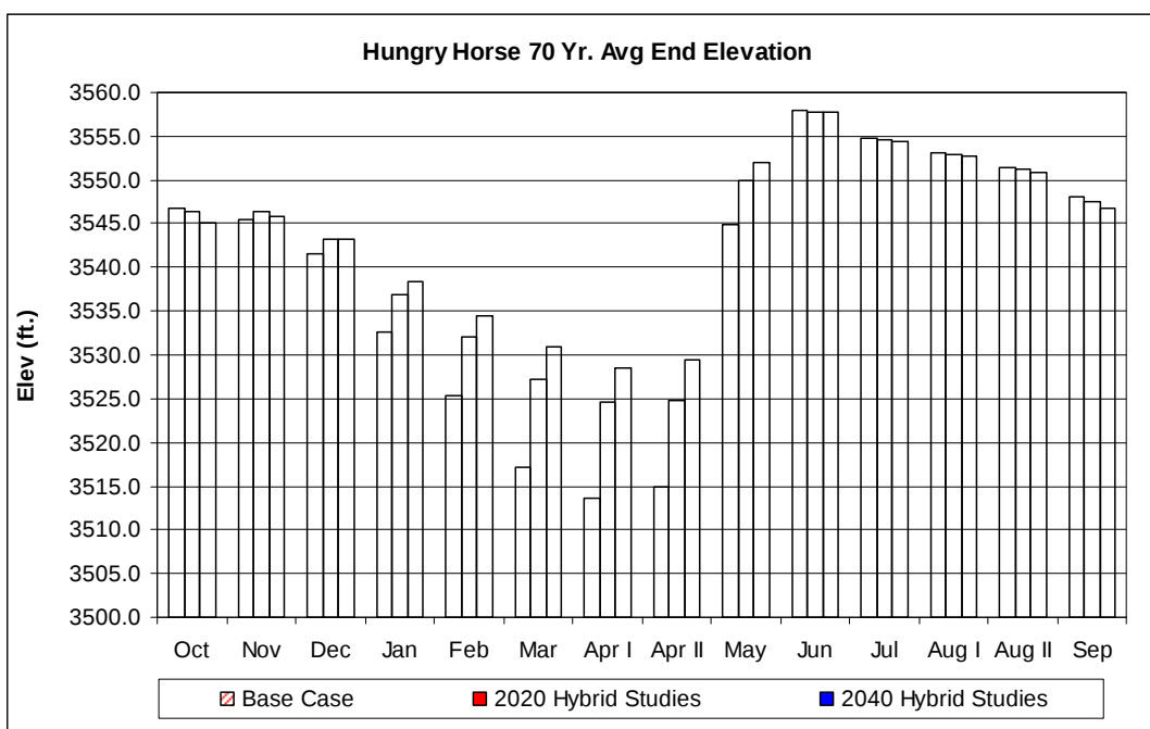
Figure 92. Hungry Horse Average End Elevation for Base Case and Climate Change Scenarios.
