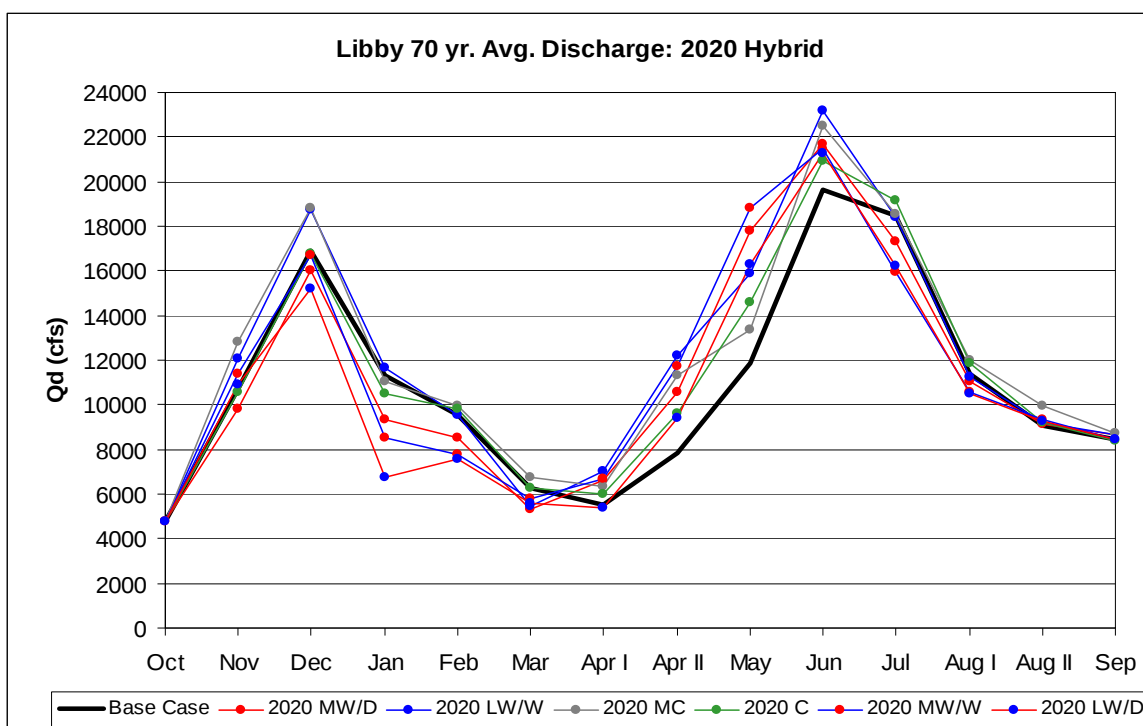
Figure 81. Libby Discharge: 2020s HD.
