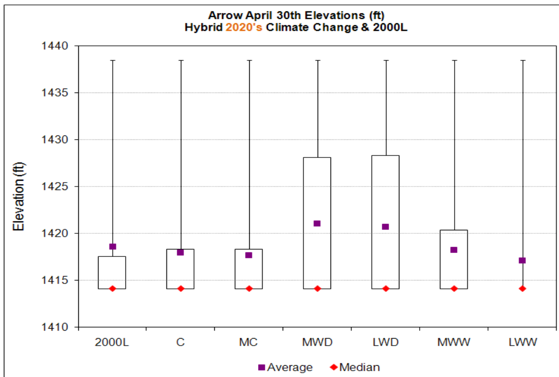
Figure 32. Arrow April 30th Elevations, 2000 Level & Climate Change Scenarios – Hybrid-Delta 2020s.
