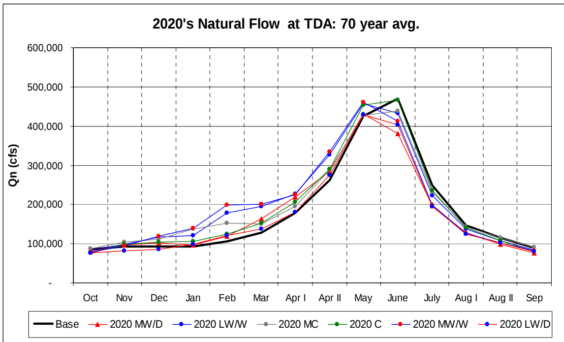
Figure 10. Monthly Seventy-year Average (1929 - 1998) Stream Flow at TDA for 2000L Modified Flows (Base) and the Six Scenarios from the 2020 Set.
