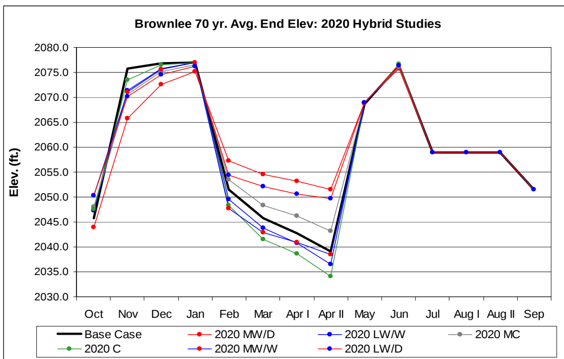
Figure 115. Brownlee period ending elevation for each 2020 Hybrid-Delta climate change scenario.
