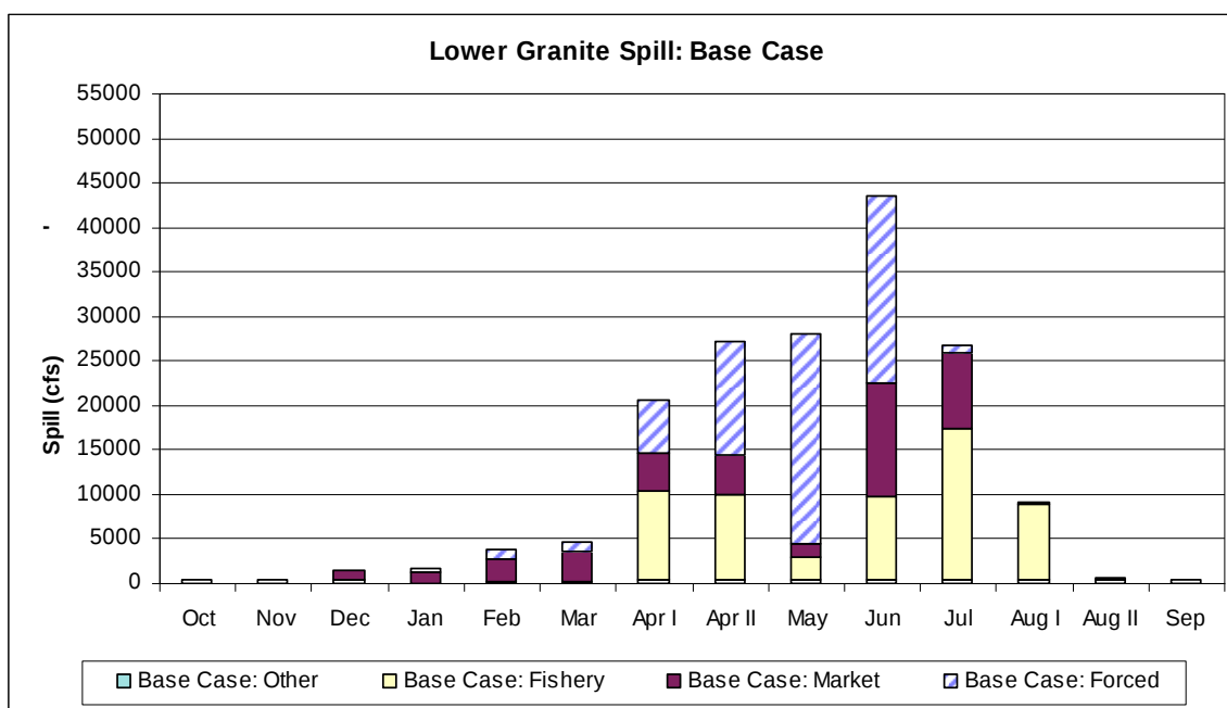
Figure 151. Base Case Lower Granite Spill Breakdown.
