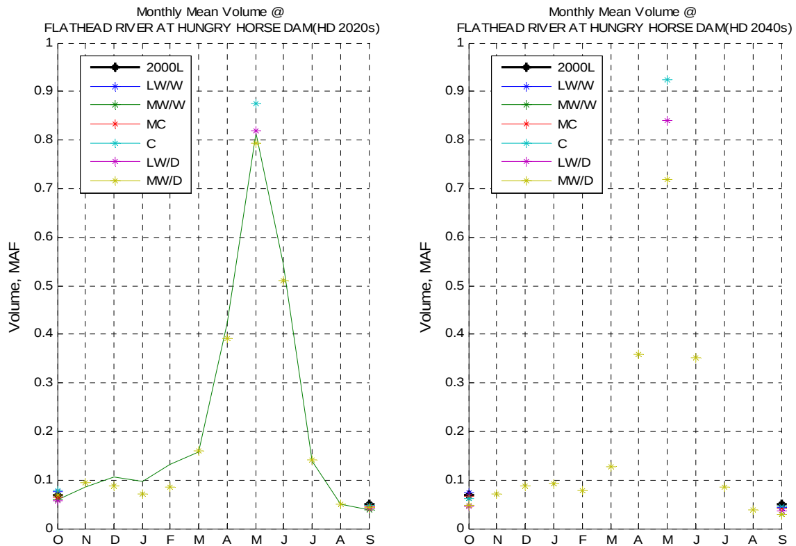
Figure 53. Hungry Horse Mean Monthly Volume – Hybrid-Delta.
