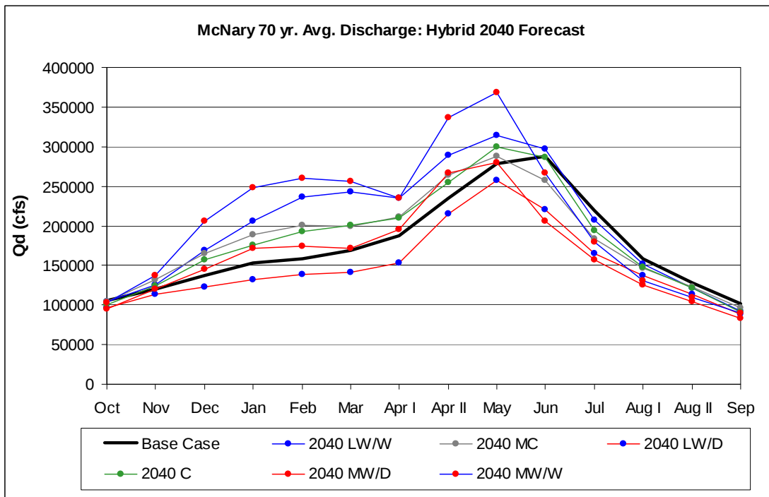
Figure 127. McNary Discharge: Hybrid-Delta 2040s
