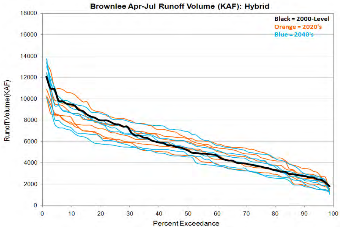
Figure 40. Brownlee Apr-Jul Runoff Volume Exceedance – Hybrid-Delta.
