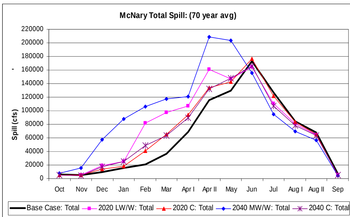
Figure 150. McNary Spill Comparison.
