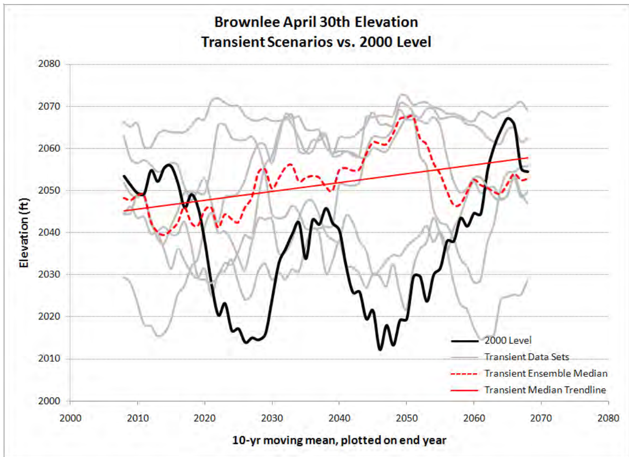
Figure 45. Brownlee April 30th Elevations Rolling Average – Transient.
