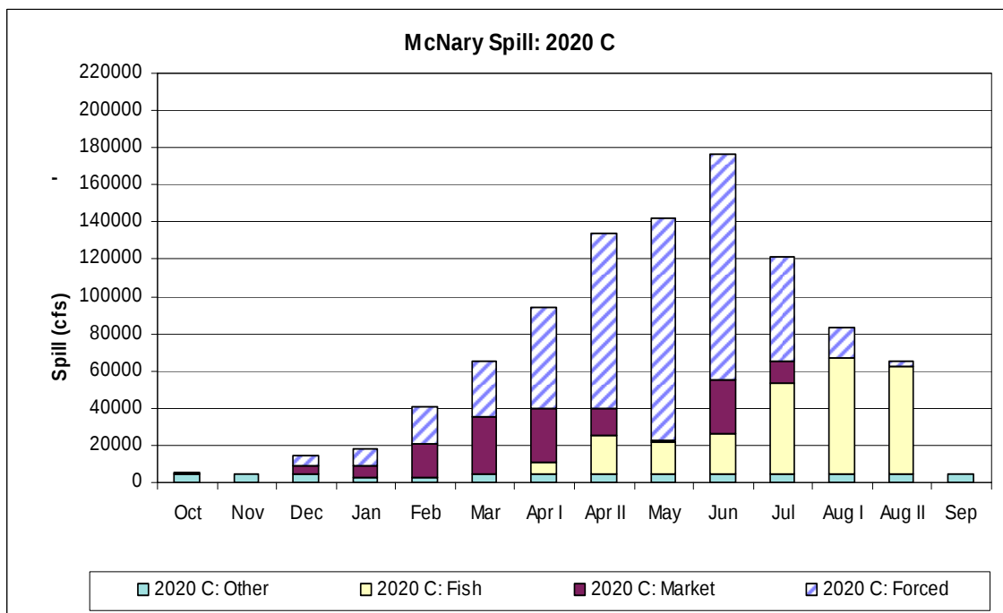
Figure 155. 2020 C Scenario: McNary Spill Breakdown.
