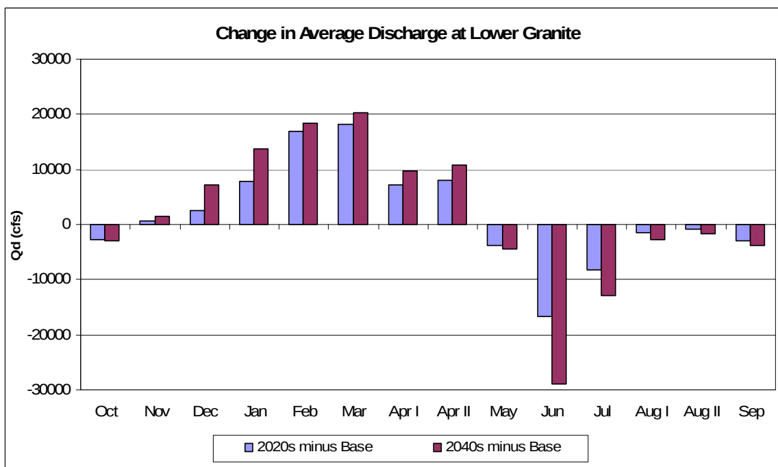
Figure 120. Lower Granite Avg. Mo. Discharge Delta for Base Case and Hybrid-Delta Scenarios.
