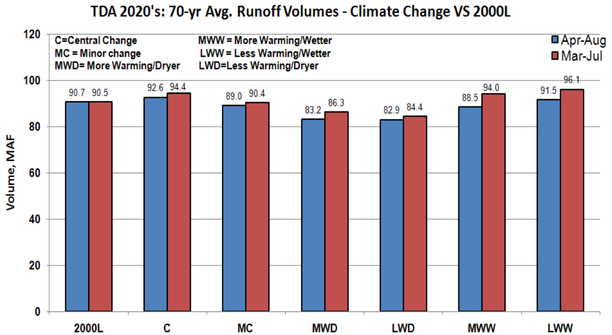
Figure 25. The Dalles Apr-Aug and Mar-Jul Runoff Volume (in kaf) – Hybrid-Delta 2020s.
