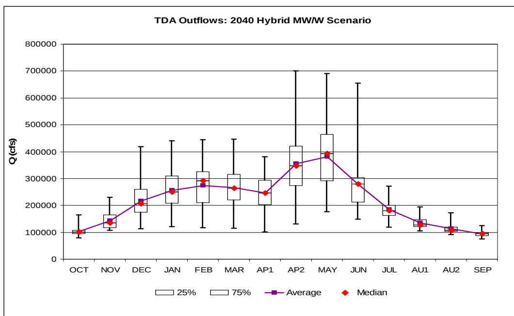
Figure 130. The Dalles Outflows for Hybrid-Delta 2040 MW/W Scenario.
