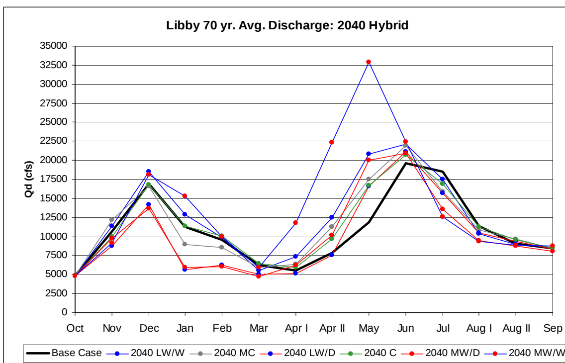
Figure 83. Libby Discharge: 2040s HD.
