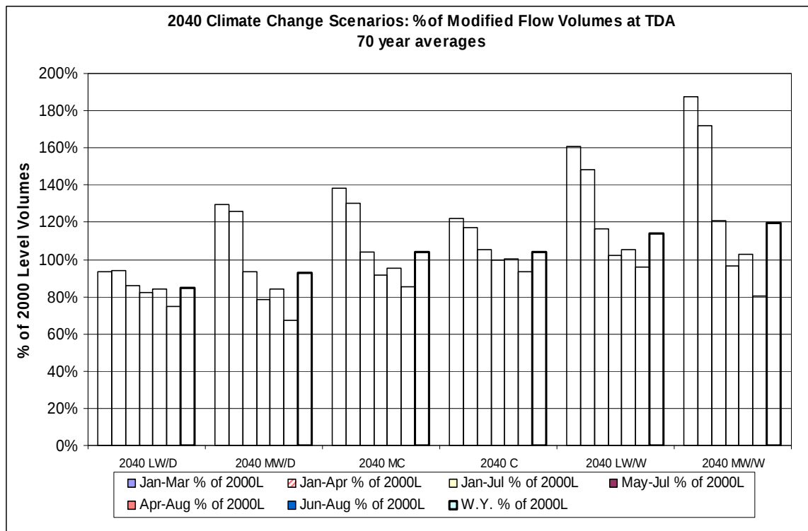
Figure 14. Six 2040 Scenarios Flow Volumes over Various Periods at TDA as Percentages of 2000L Modified Flow Volume over the Same Periods.
