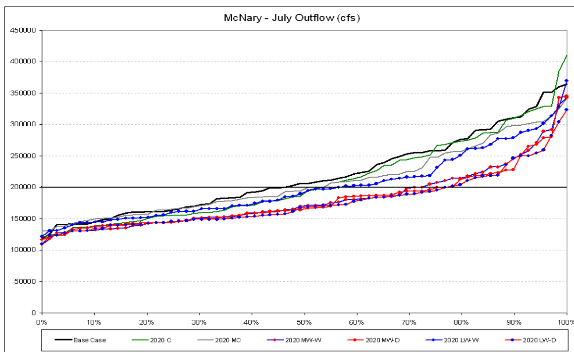
Figure 131. Comparison of Hybrid-Delta 2020 scenarios - July McNary outflow distributions.
