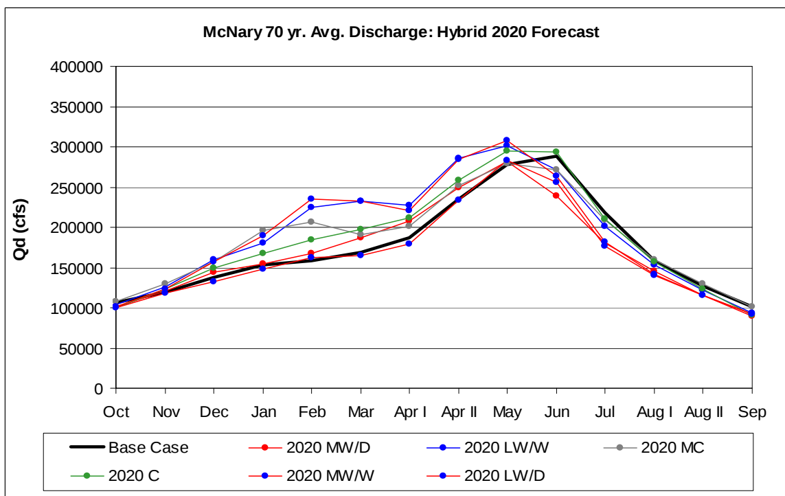
Figure 126. McNary Discharge: Hybrid-Delta 2020s
