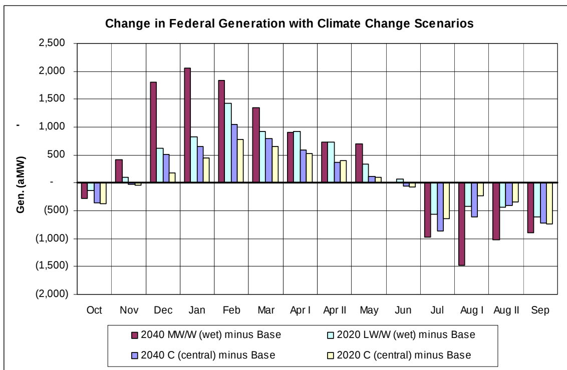
Figure 161. Climate Change Average Changes in Federal Generation.
