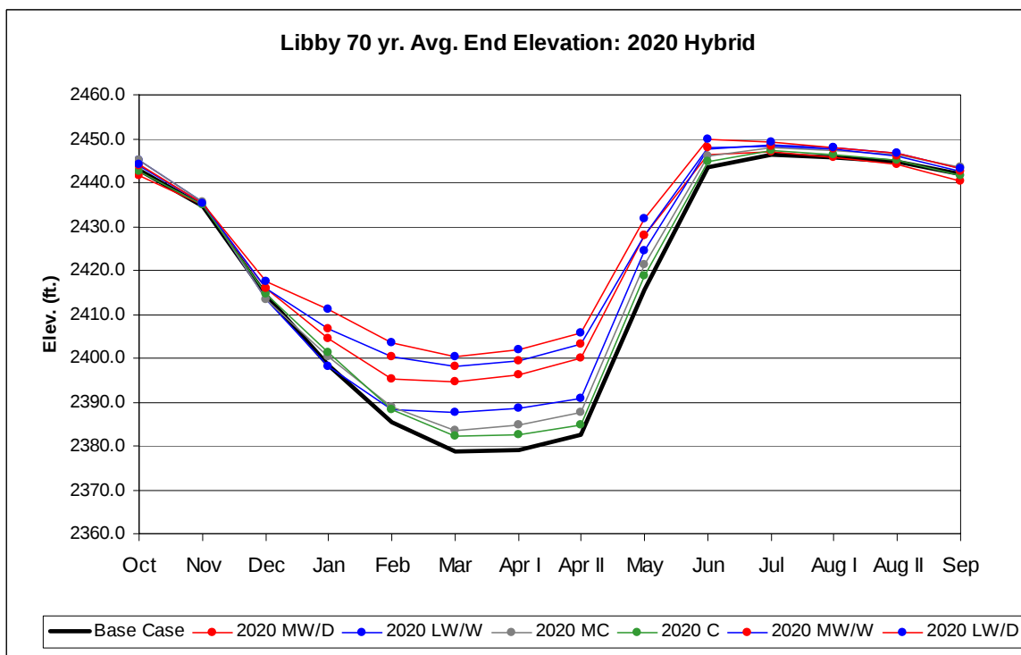
Figure 82. Libby End Elevations: 2020s HD.
