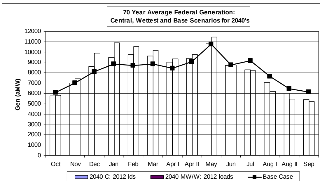
Figure 158. Federal Generation Comparison for Hybrid-Delta 2040s.
