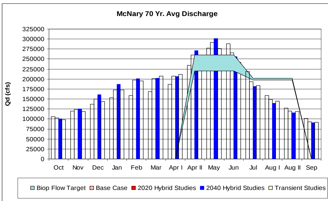
Figure 124. McNary Average Monthly Discharge for Base Case and Climate Change Scenarios.
