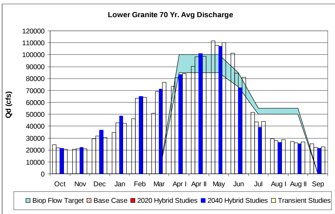
Figure 119. Lower Granite Avg. Mo. Discharge for Base Case and Climate Change Scenarios.
