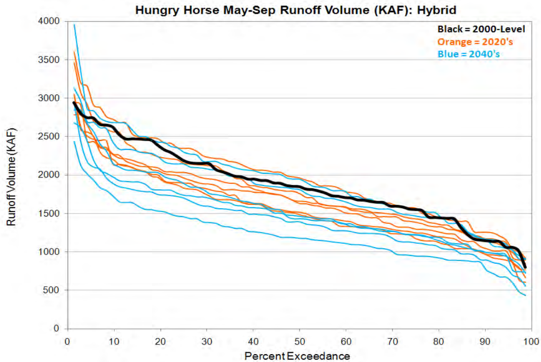
Figure 54. Hungry Horse May-Sep Runoff Volume Exceedance – Hybrid-Delta.
