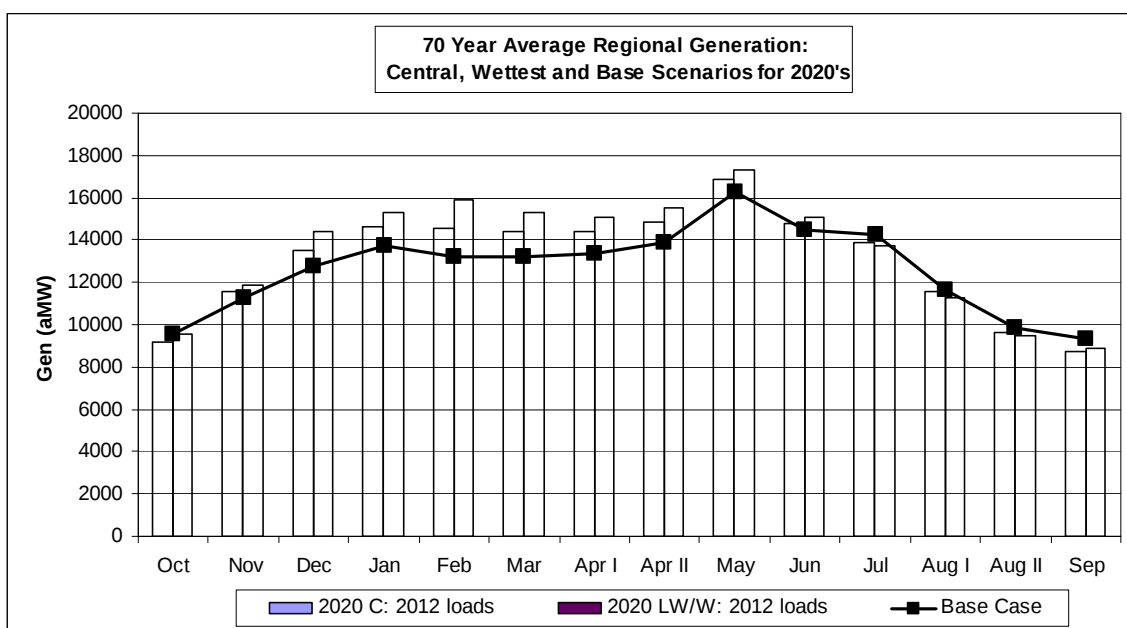
Figure 159. Regional Generation Comparison for Hybrid-Delta 2020s.
