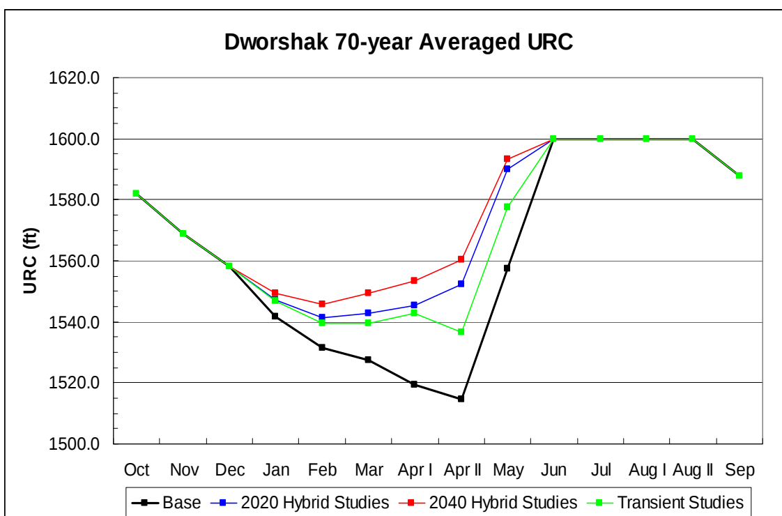
Figure 107. Dworshak seventy-year averaged URC for Base Case and Climate Change Scenarios.
