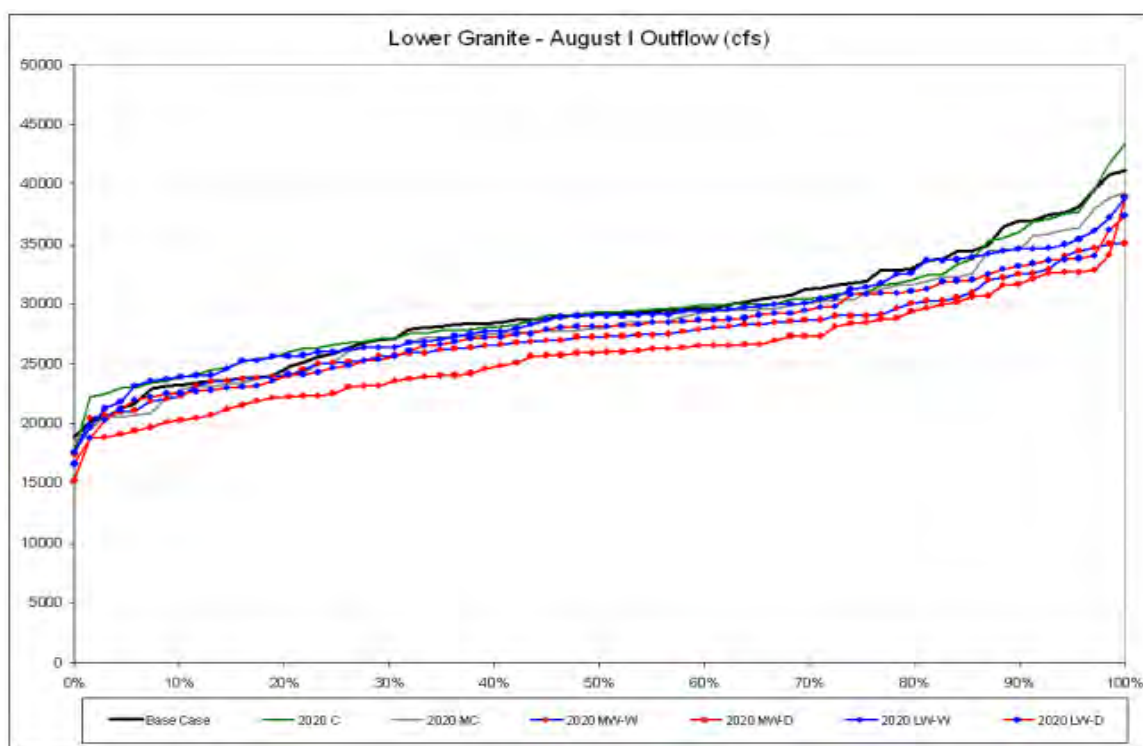
Figure 138. Comparison of 2020 Hybrid-Delta scenarios - August I Lower Granite outflow distributions.
