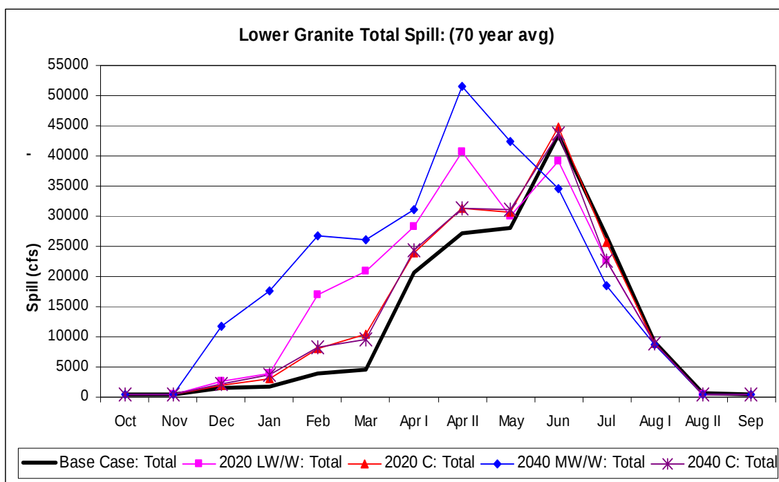
Figure 149. Lower Granite Spill Comparison.
