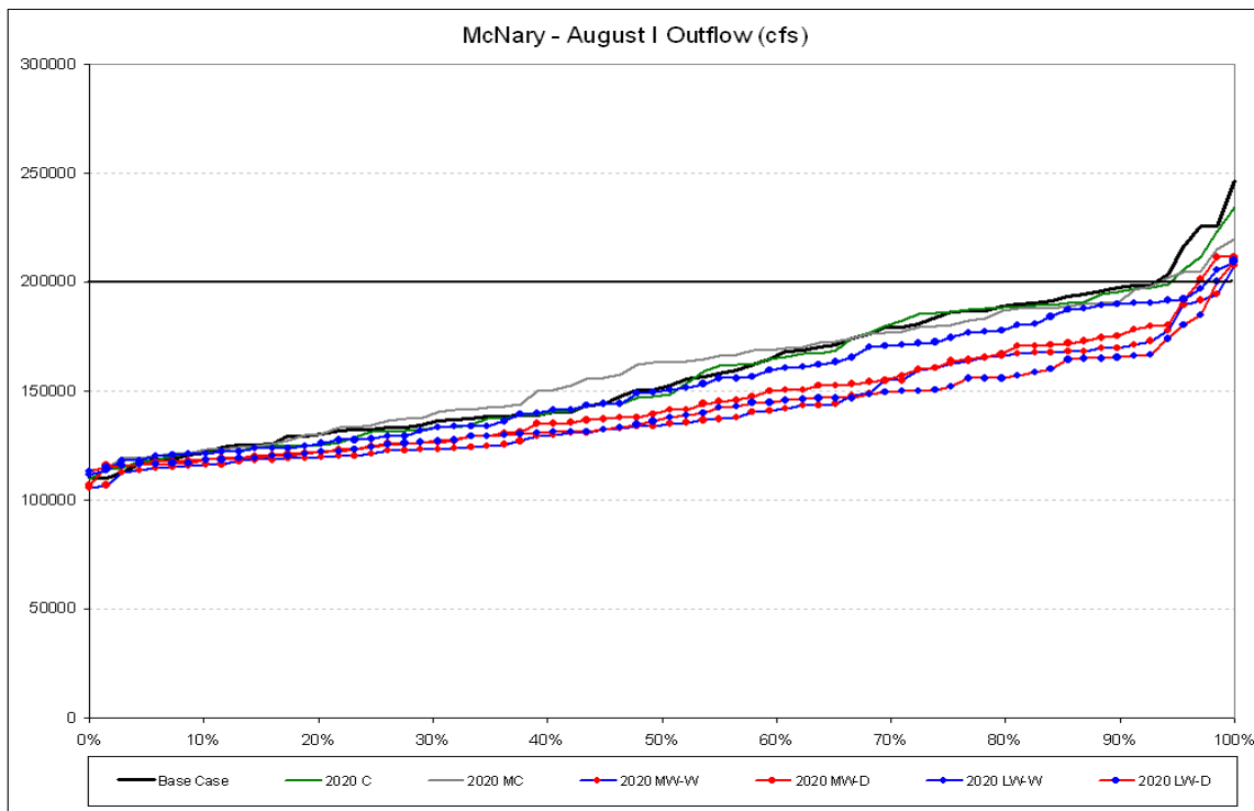
Figure 132. Comparison of Hybrid-Delta 2020 scenarios - August I McNary outflow distributions.
