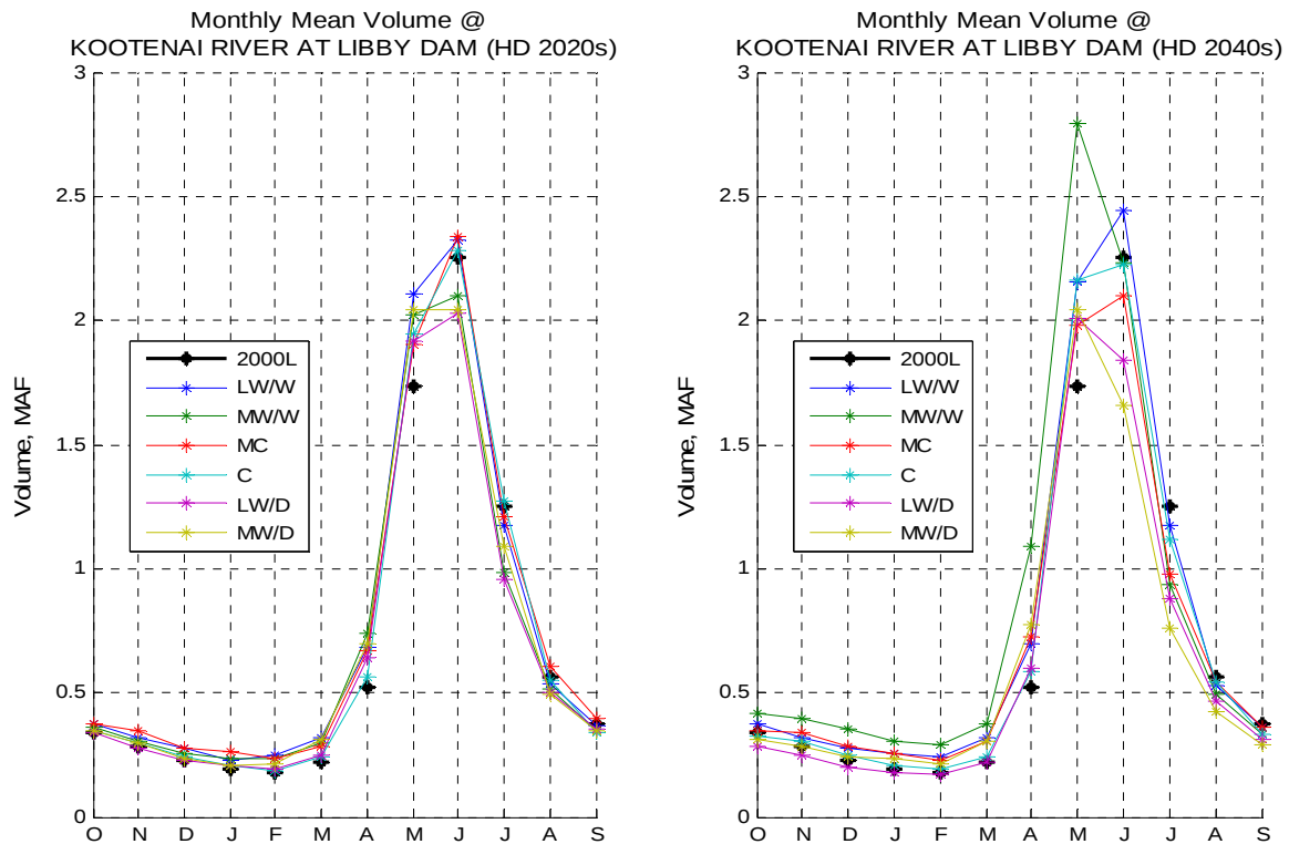
Figure 46. Libby Mean Monthly Volume – Hybrid-Delta.
