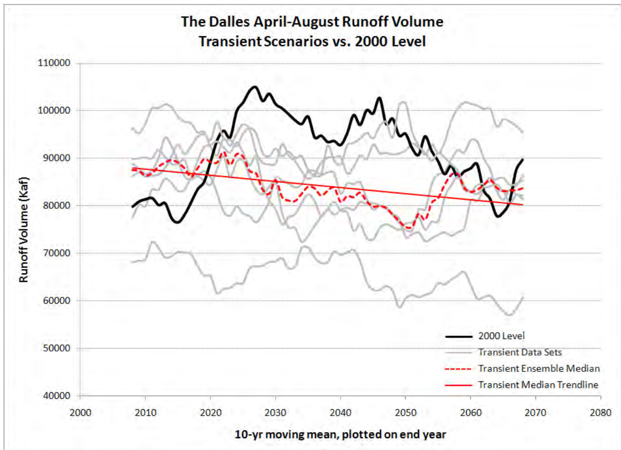
Figure 24. The Dalles Apr-Aug Runoff Volume Rolling Average – Transient.
