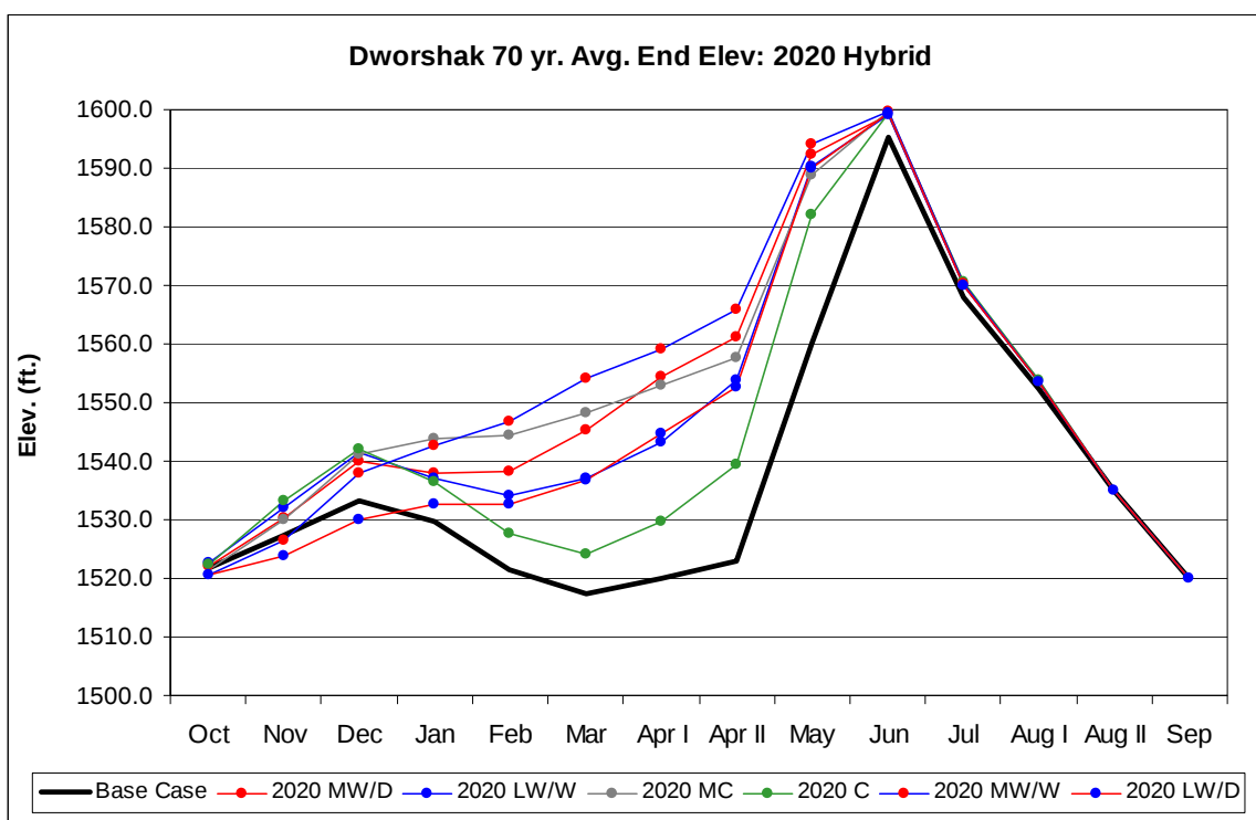
Figure 110. Dworshak End Elevations: 2020s HD.
