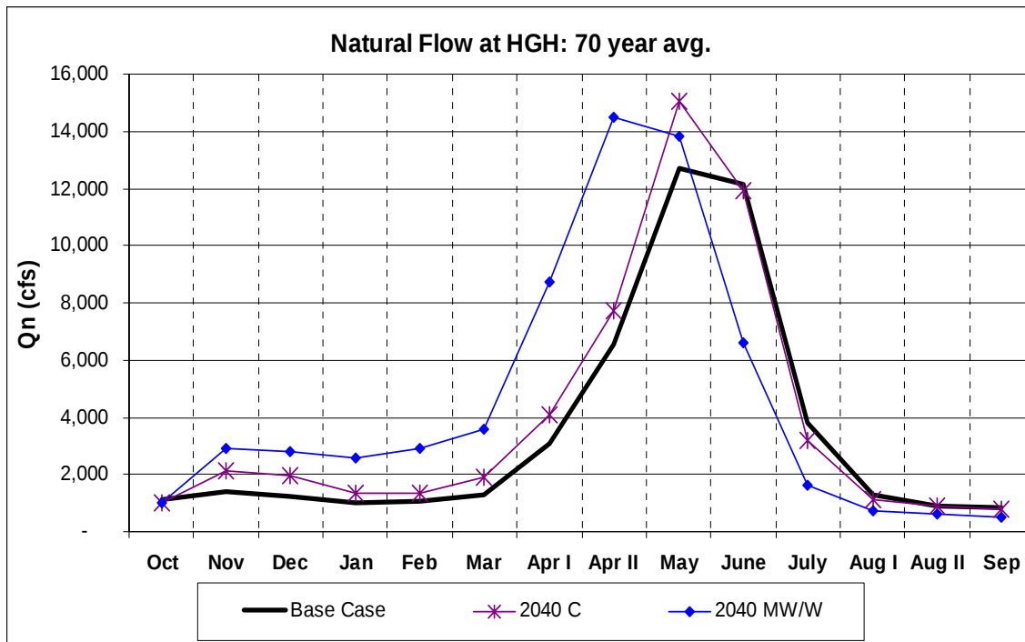
Figure 146. Hungry Horse Natural Inflows for 2040s.
