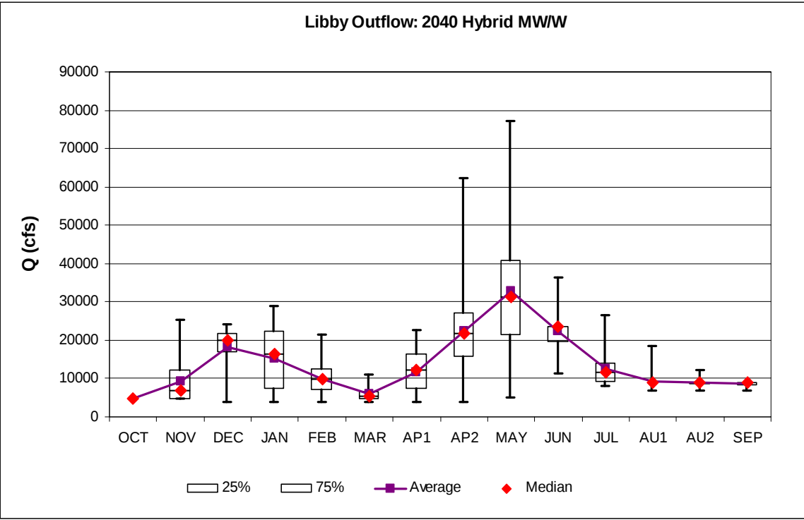
Figure 89. Libby 70 year outflow distribution for 2040 Hybrid-Delta MW/W study.
