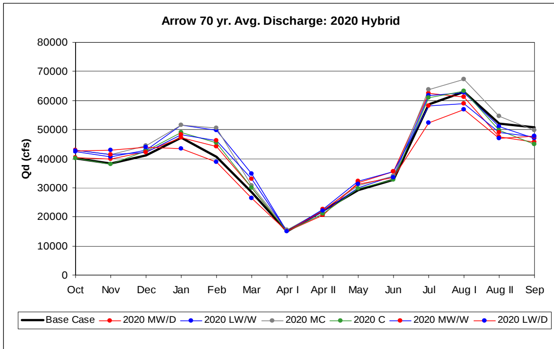
Figure 75. Arrow Discharge: 2020 Hybrid-Delta.
