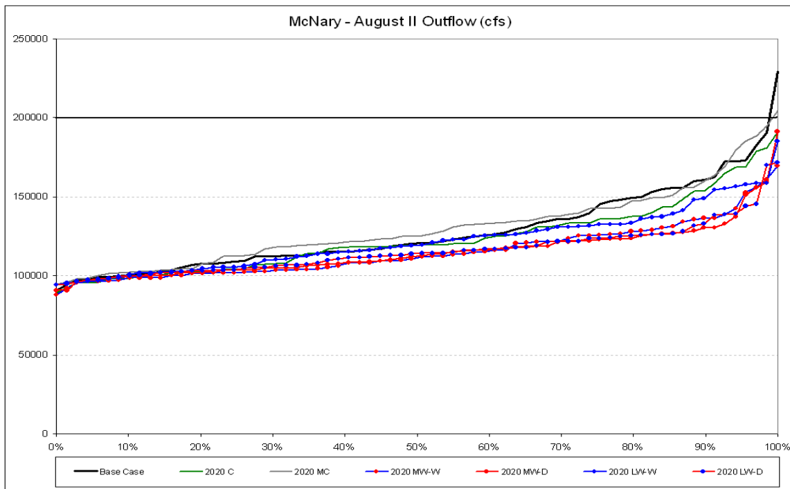
Figure 133. Comparison of Hybrid-Delta 2020 scenarios - August II McNary outflow distributions.
