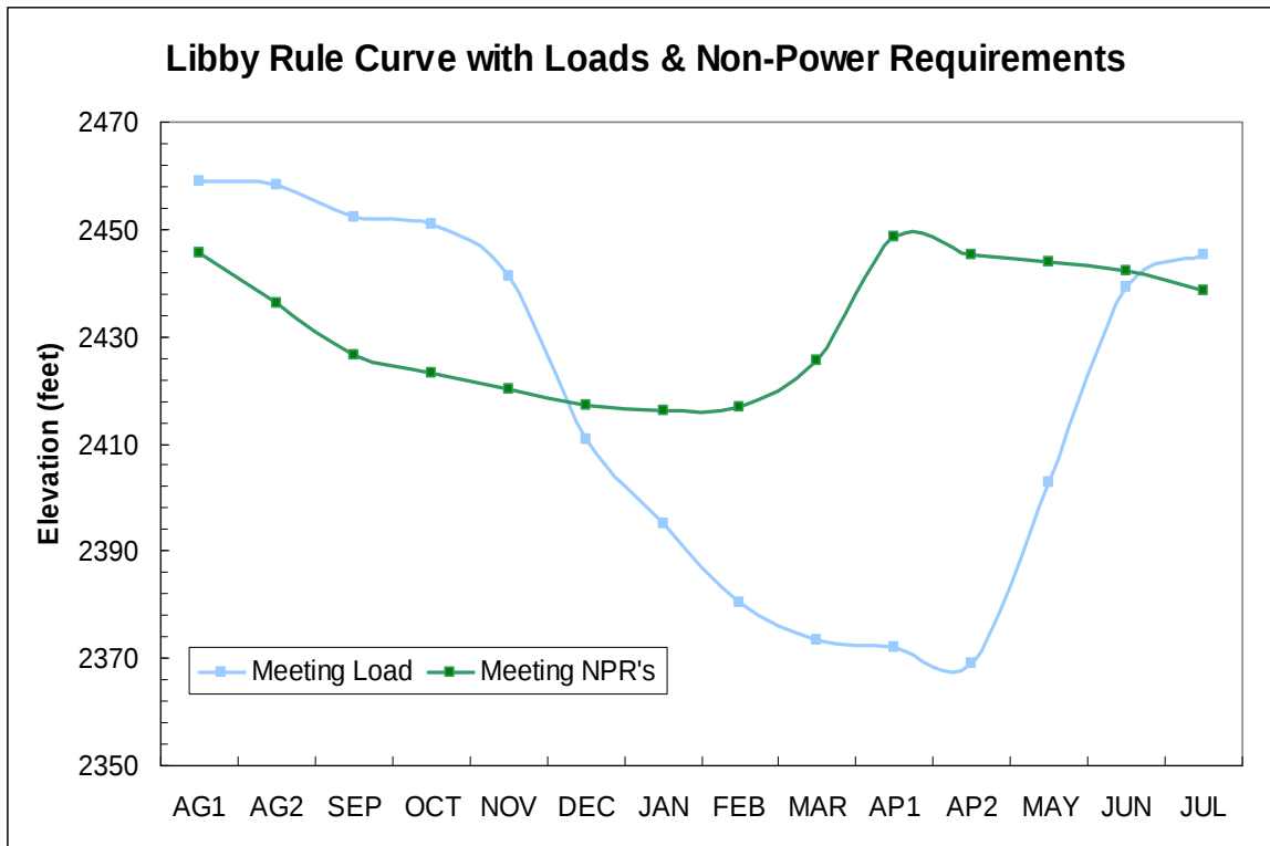
Figure 72. Libby Rule Curve for FELCC and NPRs
