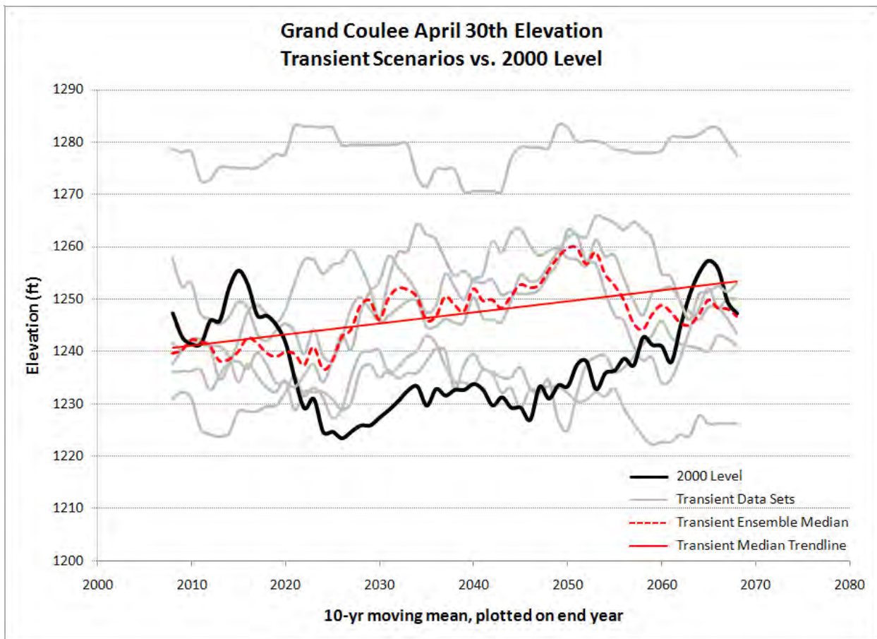
Figure 38. Grand Coulee April 30th Elevations Rolling Average – Transient.
