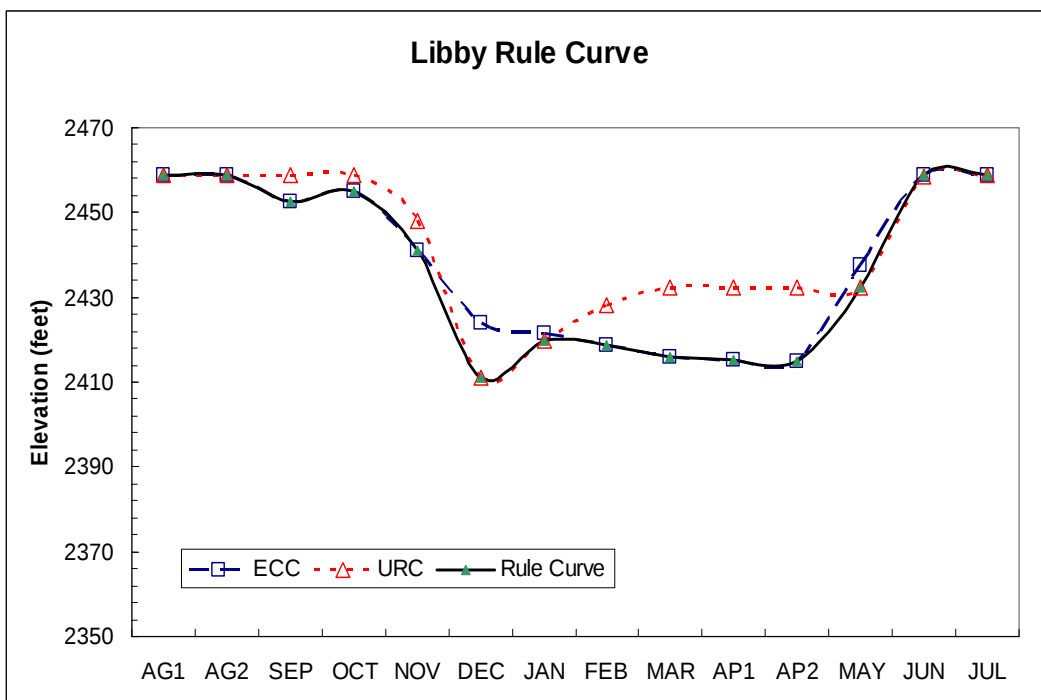
Figure 70. Comparison between Libby ECC, URC and Operating Rule Curve.
