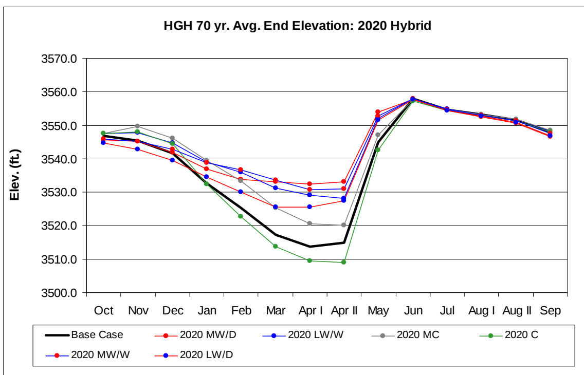
Figure 95. Hungry Horse End Elevations: 2020s HD.
