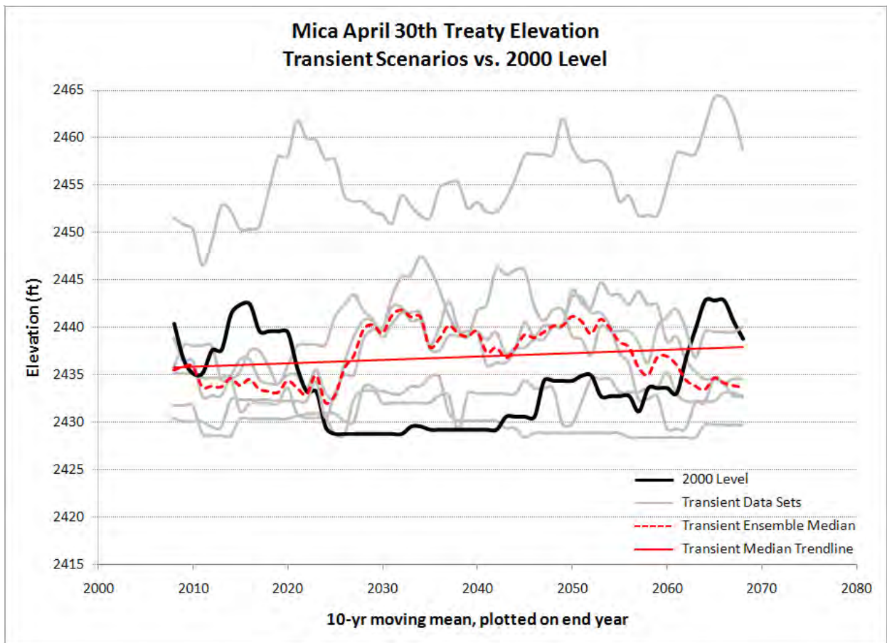
Figure 30. Mica April 30th Treaty Elevations Rolling Average – Transient.
