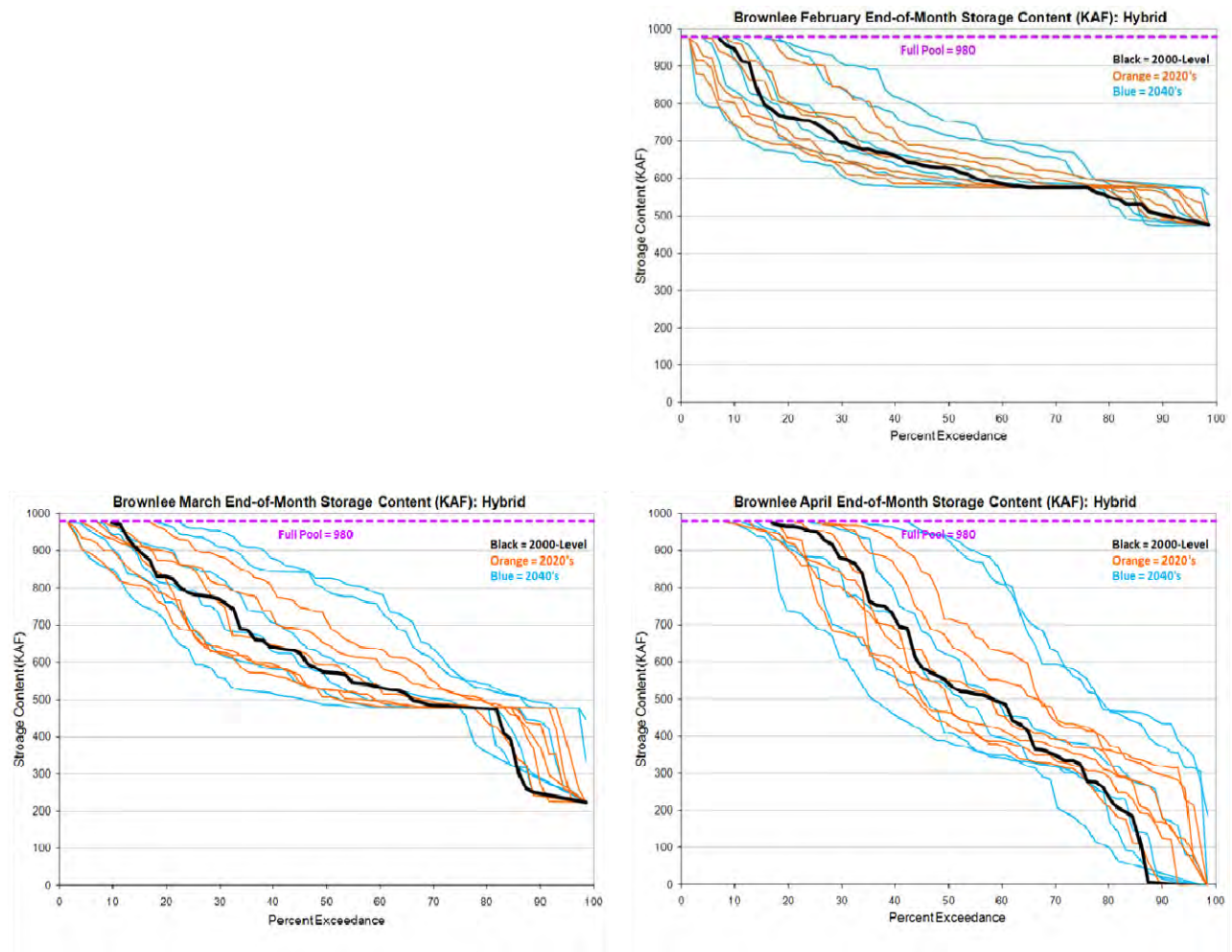
Figure 42. Brownlee Flood Control Storage Exceedance – Hybrid-Delta.
