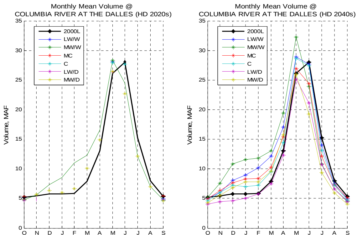
Figure 22. The Dalles Mean Monthly Volume – Hybrid-Delta.
