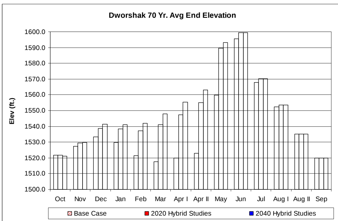
Figure 106. Dworshak Average End Elevation for Base Case and Climate Change Scenarios.
