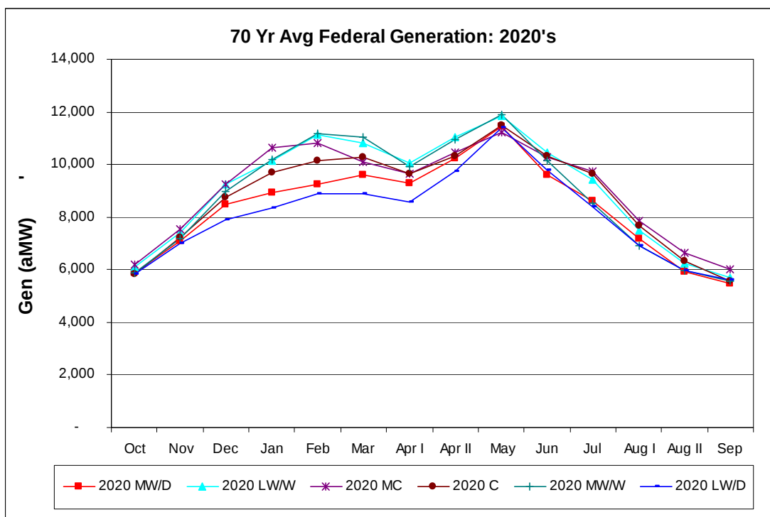
Figure 163. Federal Generation for Hybrid-Delta 2020s Scenarios.
