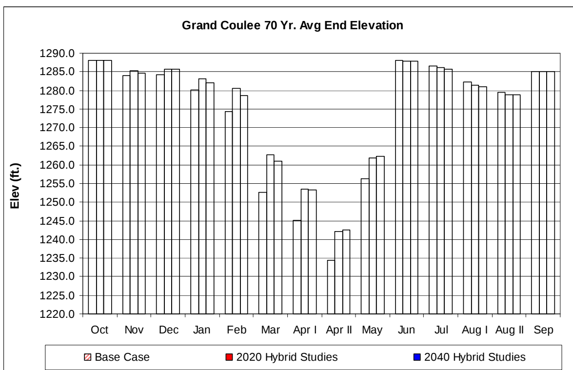
Figure 99. Grand Coulee Average End Elevation for Base Case and Climate Change Scenarios.
