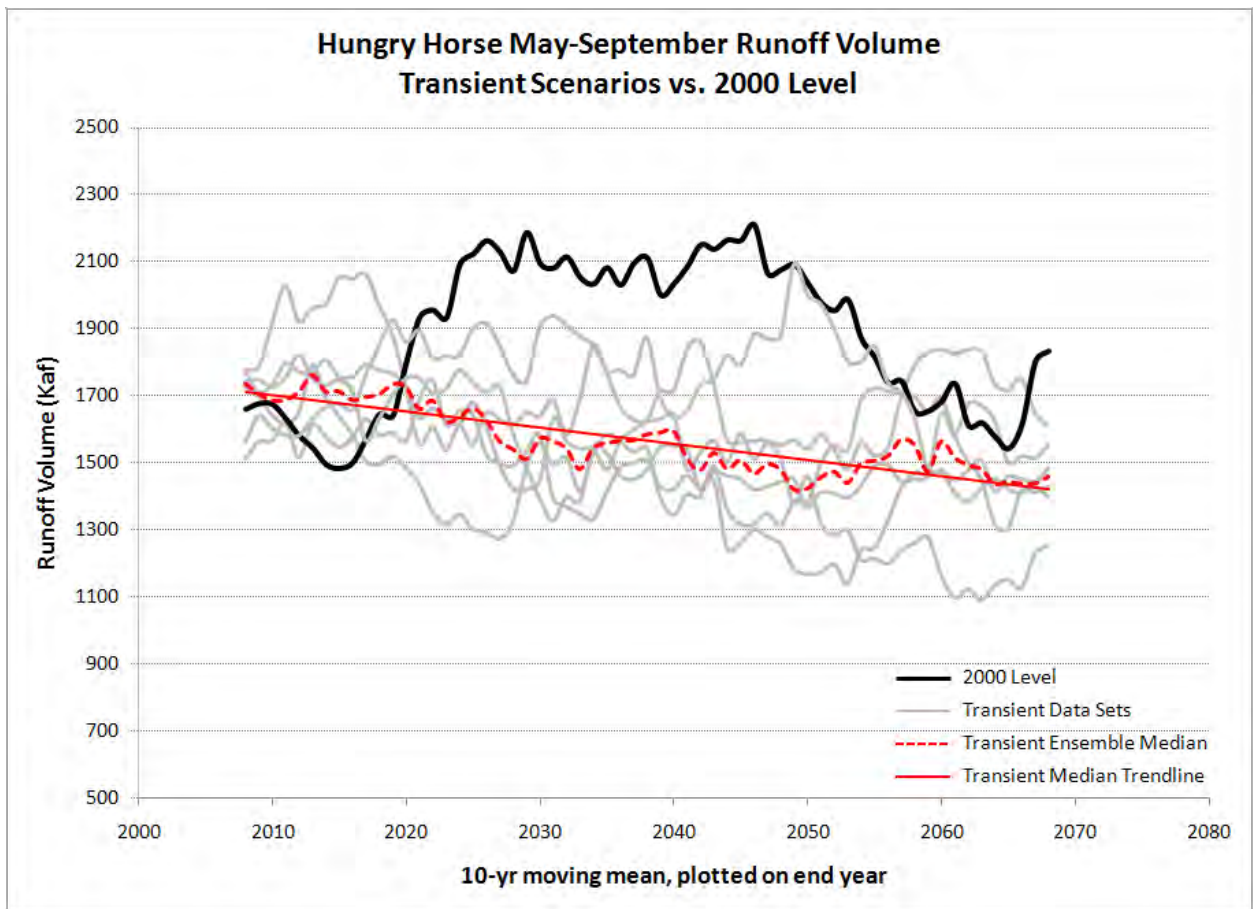
Figure 55. Hungry Horse May-Sep Runoff Volume Rolling Average – Transient.
