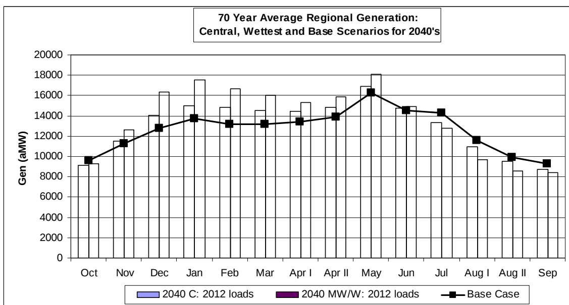
Figure 160. Regional Generation Comparison for Hybrid-Delta 2040s.
