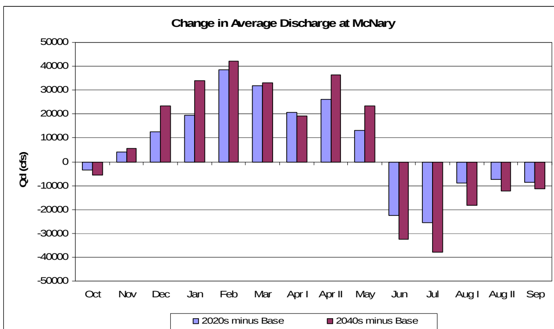
Figure 125. McNary Avg. Mo. Discharge Delta for Base Case and Hybrid-Delta Climate Change Scenarios.
