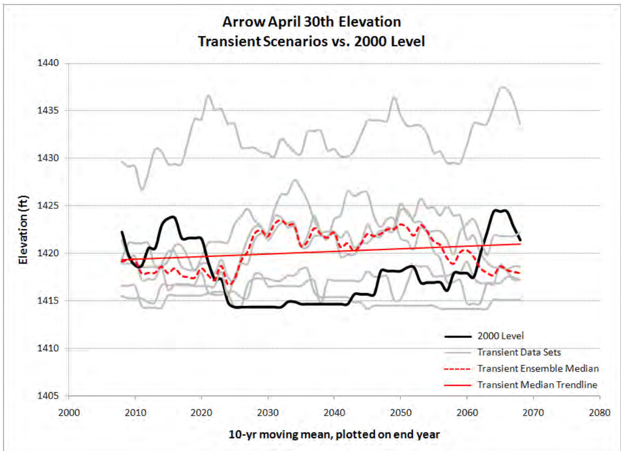
Figure 34. Arrow April 30th Elevations Rolling Average – Transient.
