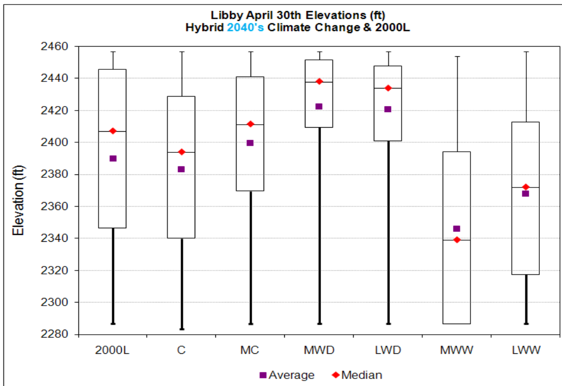
Figure 51. Libby April 30th Elevations, 2000 Level & Climate Change Scenarios – Hybrid-Delta 2040s.
