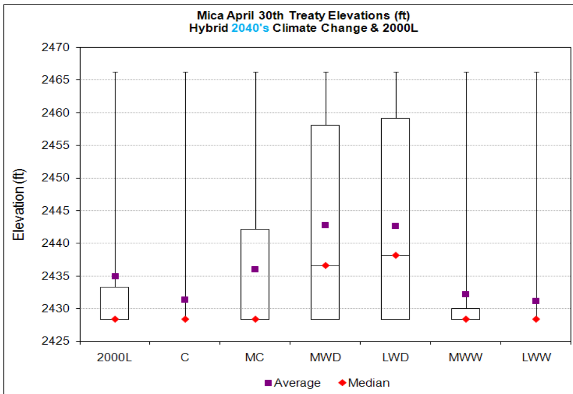
Figure 29. Mica April 30th Treaty Elevations – Hybrid-Delta 2040s.
