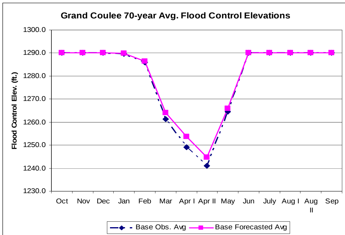
Figure 16. Grand Coulee URCs for Forecasted and Observed Volumes
