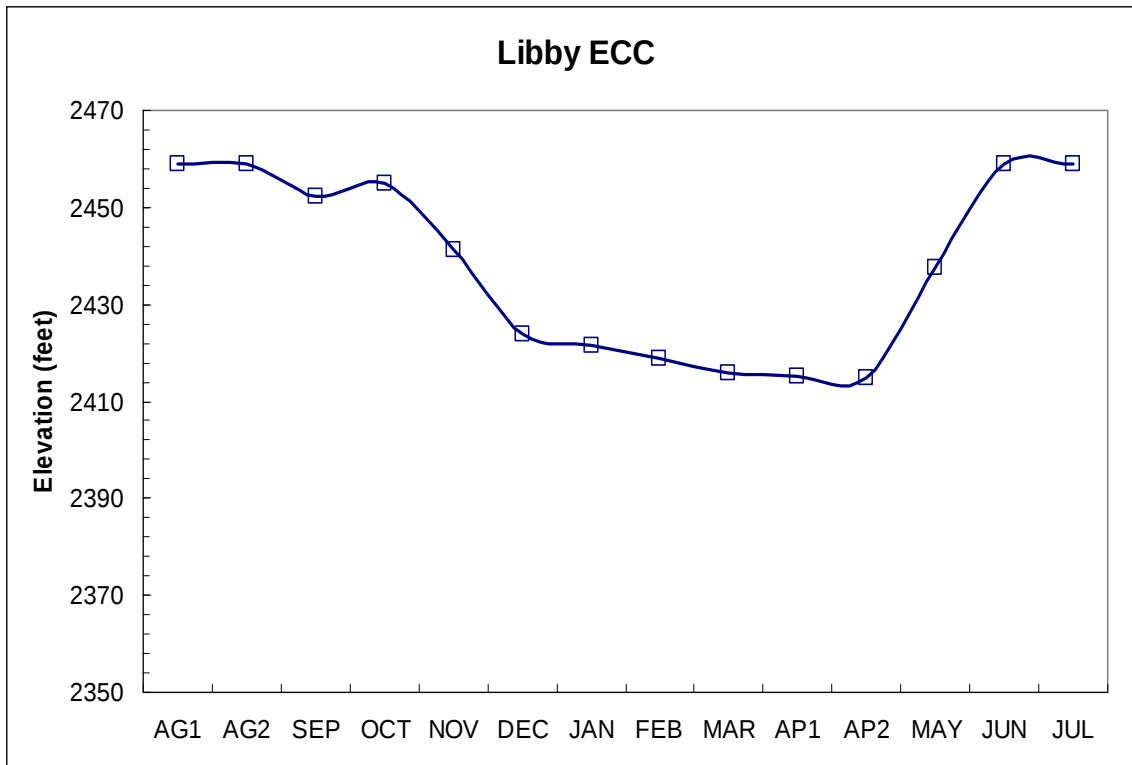
Figure 68. Libby ECC for the 1937 water-year historic stream flow.
