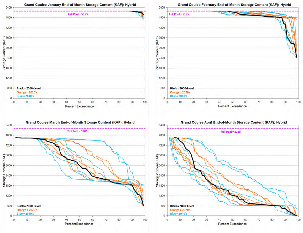
Figure 35. GCL Flood Control Storage Exceedance – Hybrid-Delta.
