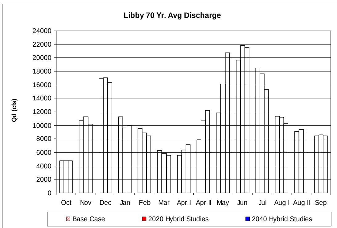
Figure 79. Libby Average Monthly Discharge for Base Case and Climate Change Scenarios.
