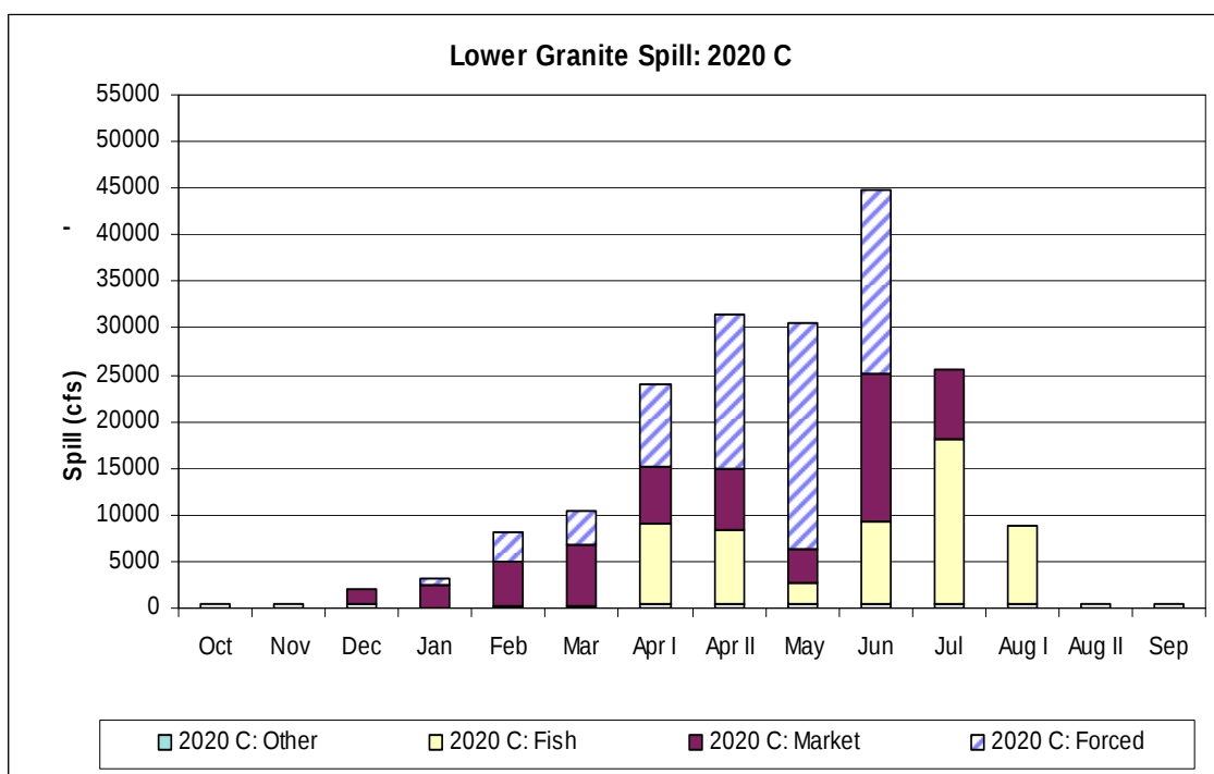
Figure 152. 2020 C Scenario: Lower Granite Spill Breakdown.
