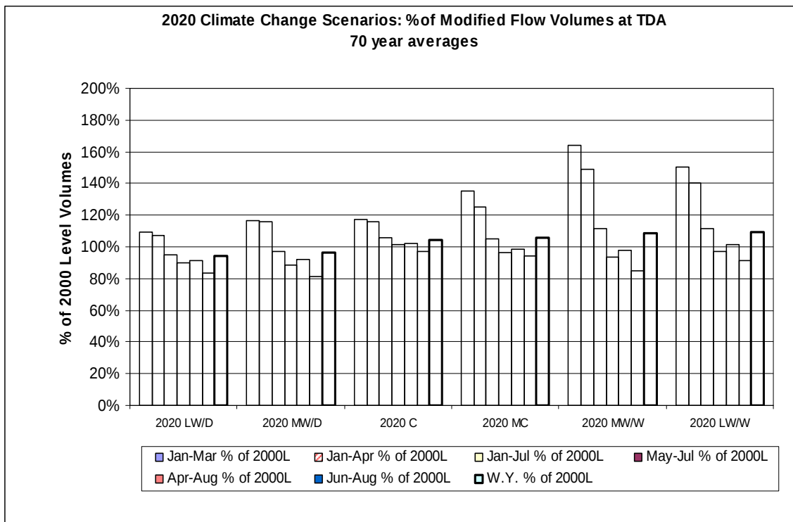
Figure 13. Six 2020 Scenarios Flow Volumes over Various Periods at TDA as Percentages of 2000L Modified Flow Volume over the Same Periods.
