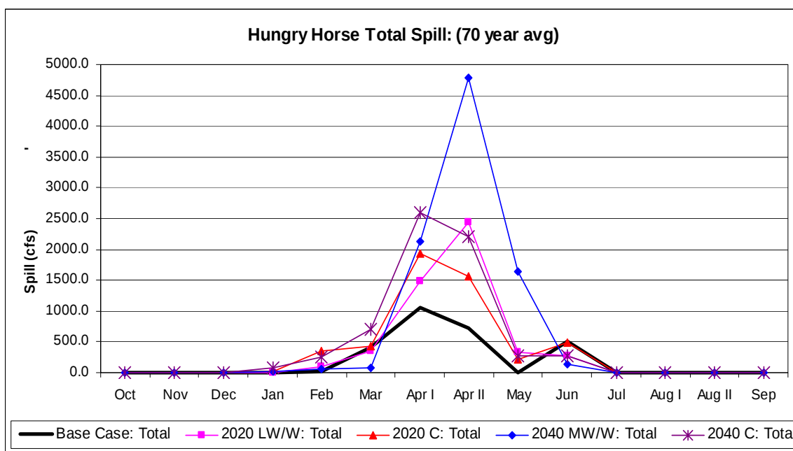
Figure 145. Hungry Horse Spill Comparison.
