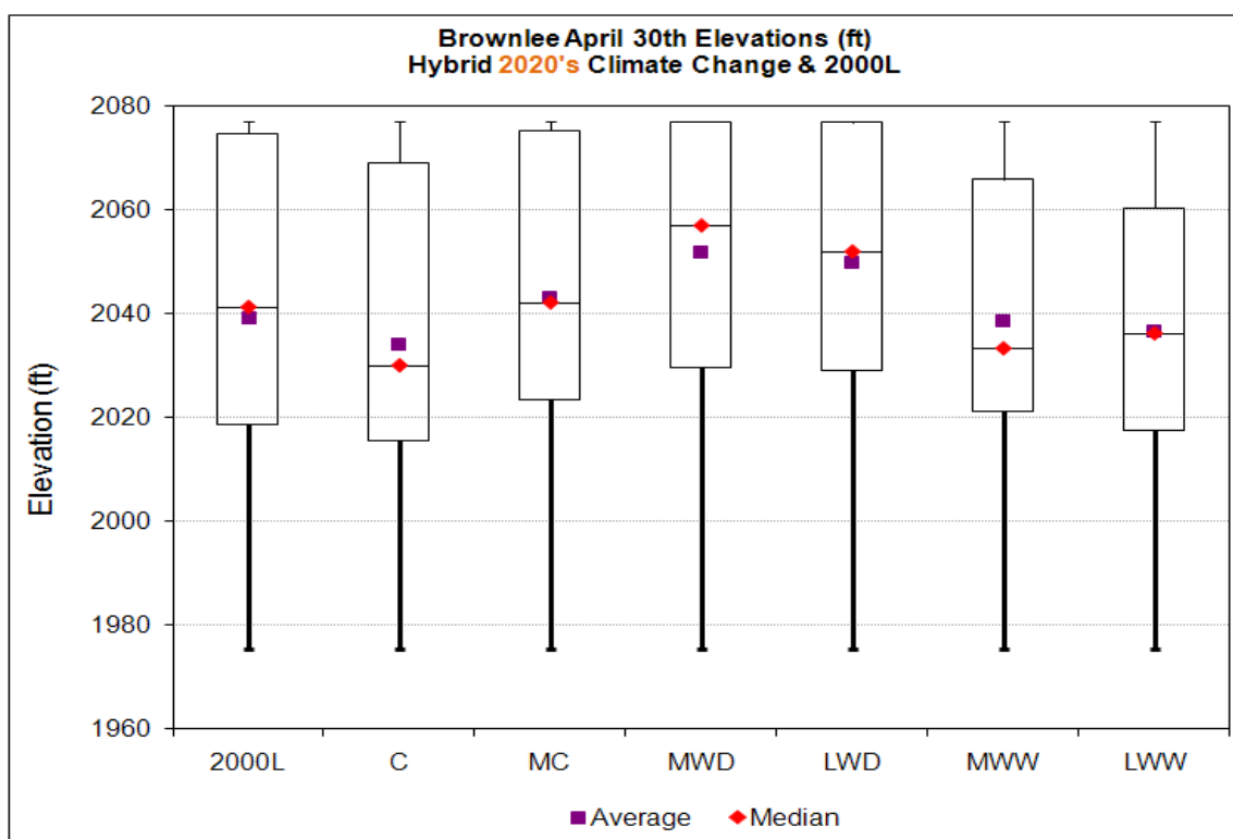
Figure 43. Brownlee April 30th Elevations, 2000 Level & Climate Change Scenarios – HD 2020s.
