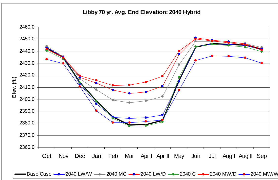
Figure 84. Libby End Elevations: 2040s HD.
