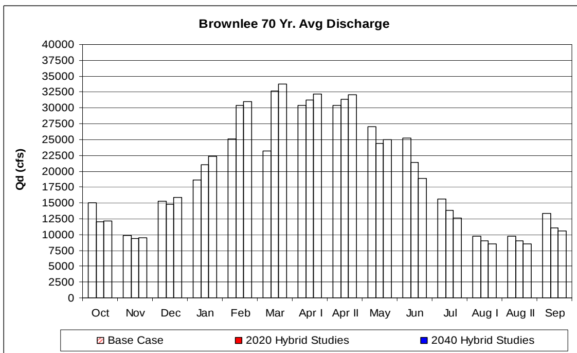
Figure 114. Comparison of month average Brownlee discharge for the Base Case, 2020 Hybrid-Delta and 2040 Hybrid-Delta climate change scenarios.
