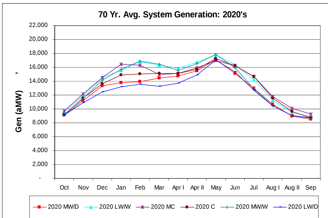
Figure 164. Regional System Generation for Hybrid-Delta 2020s Scenarios.
