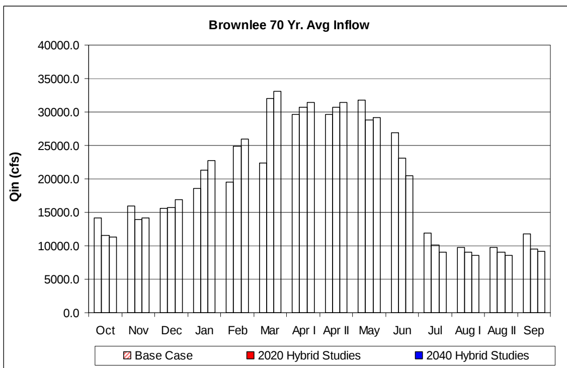
Figure 112. Comparison of month average Brownlee inflow for the Base Case, 2020 Hybrid-Delta and 2040 Hybrid-Delta climate change scenarios.
