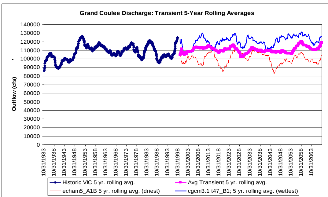
Figure 104. Coulee 5-Yr. Rolling Average Discharge for Historic and Transient Scenarios.
