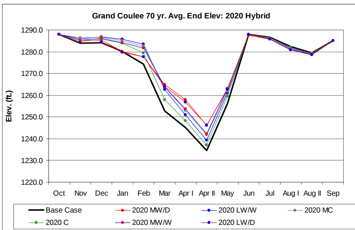
Figure 102. Grand Coulee End Elevations: 2020s HD.
