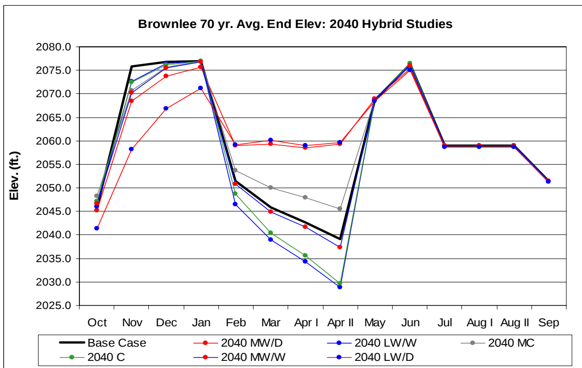
Figure 117. Brownlee period ending elevation for each 2040 Hybrid-Delta climate change scenario.
