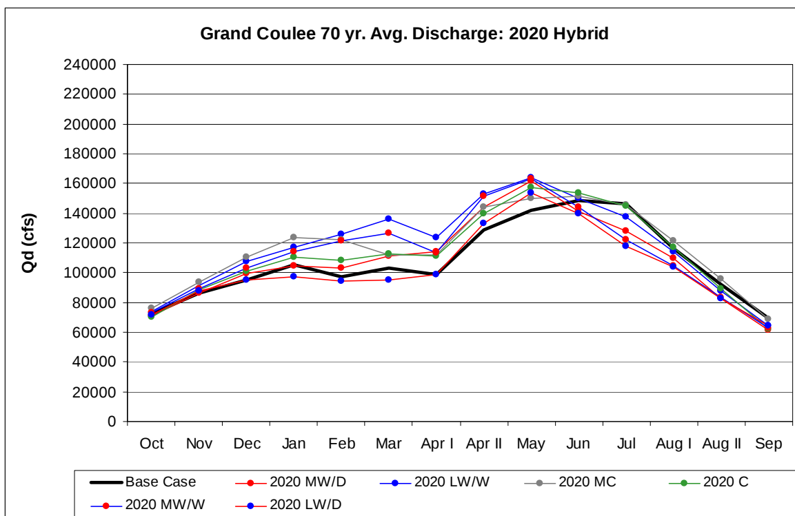
Figure 100. Grand Coulee Discharge: 2020s Hybrid-Delta.
