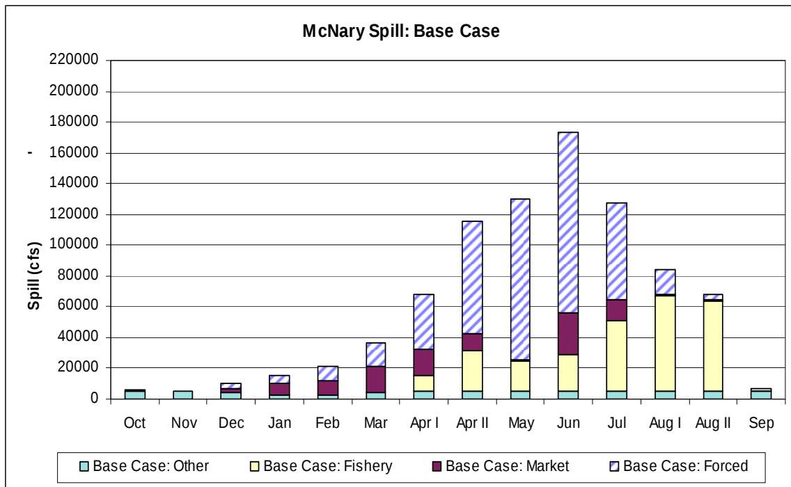
Figure 154. Base Case McNary Spill Breakdown.
