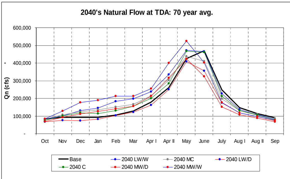
Figure 11. Monthly Seventy-year Average (1929 - 1998) Stream Flow at TDA for 2000L Modified Flows (Base Case) and the Six Scenarios from the 2040 Set.
