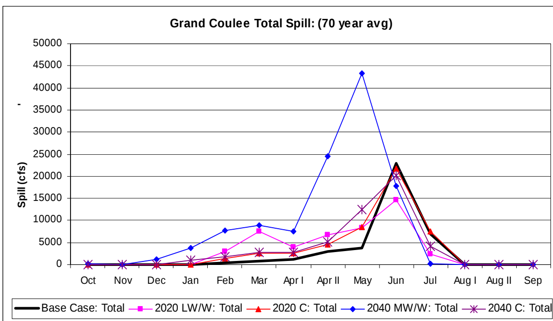
Figure 147. Grand Coulee Spill Comparison.
