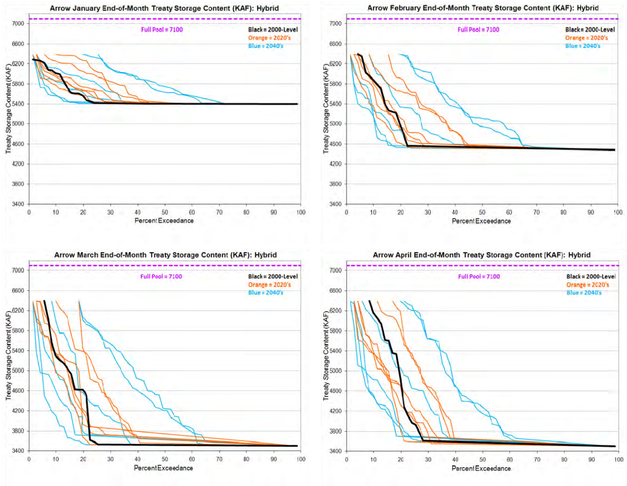
Figure 31. ARDB Flood Control Storage Exceedance – Hybrid-Delta.
