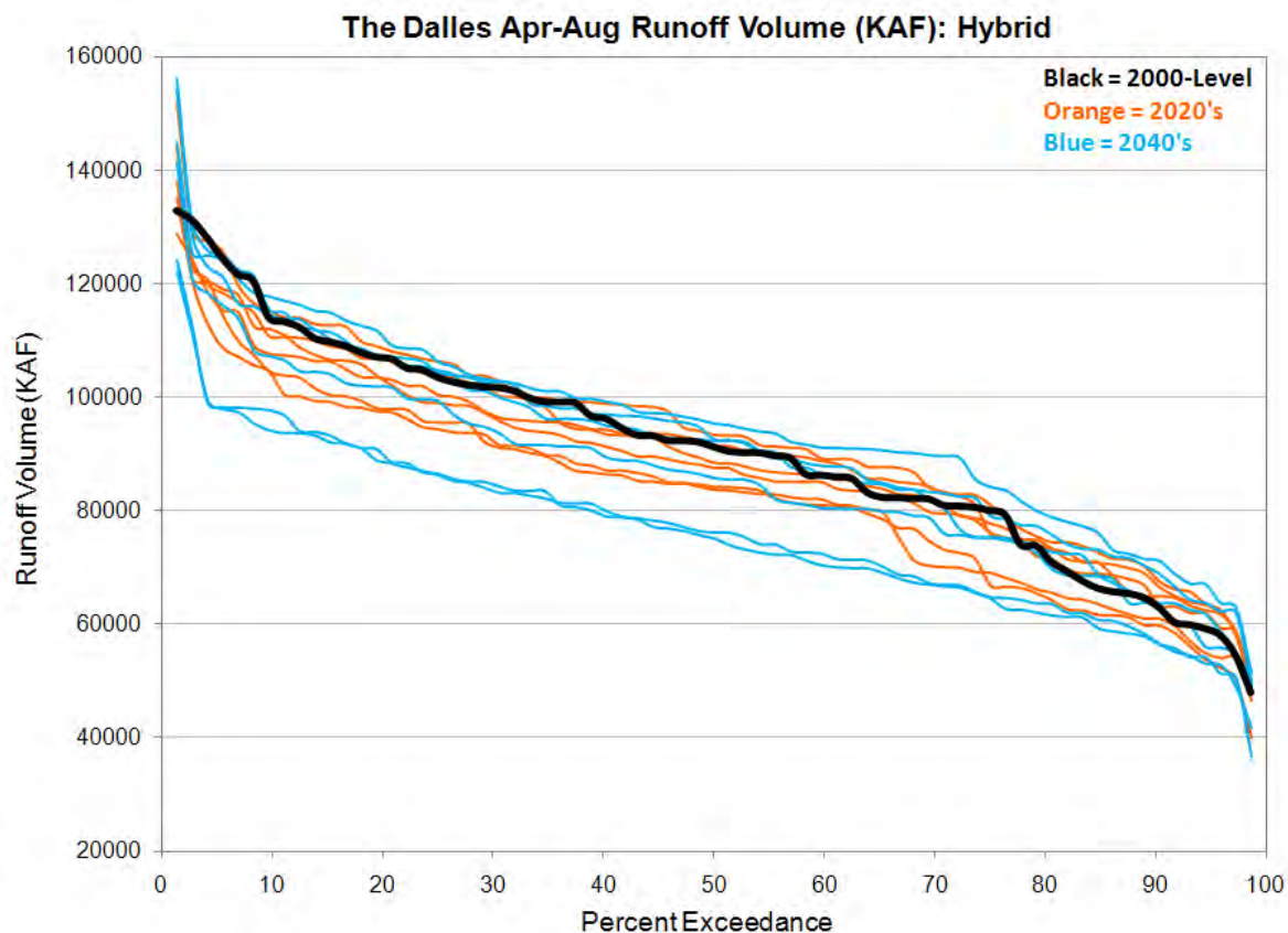
Figure 23. The Dalles Apr-Aug Runoff Volume Exceedance-Hybrid-Delta.
