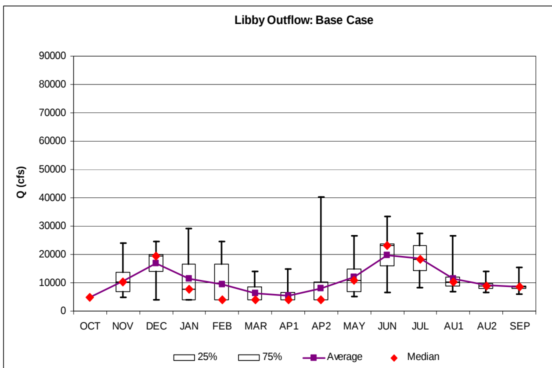
Figure 87. Libby Base Case 70 year discharge distribution.
