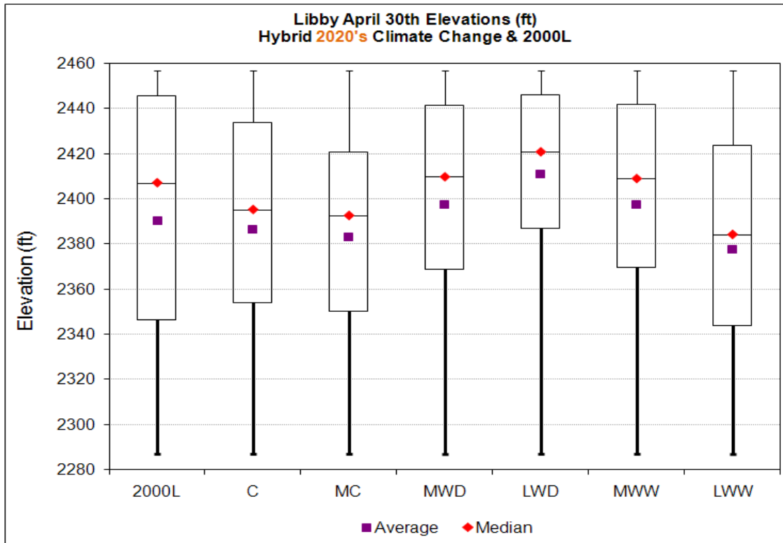
Figure 50. Libby April 30th Elevations, 2000 Level & Climate Change Scenarios – Hybrid-Delta 2020s.
