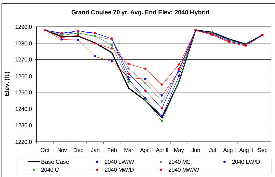
Figure 103. Grand Coulee End Elevations: 2040s HD.
