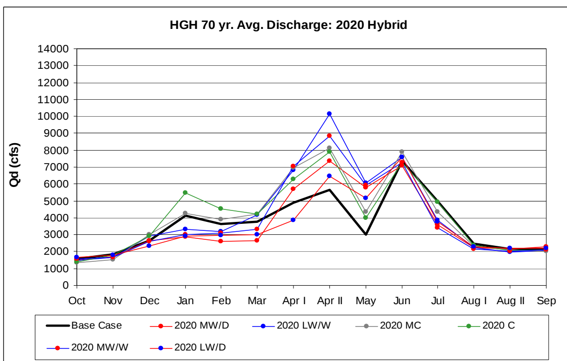
Figure 94. Hungry Horse Discharge: 2020s Hybrid-Delta.
