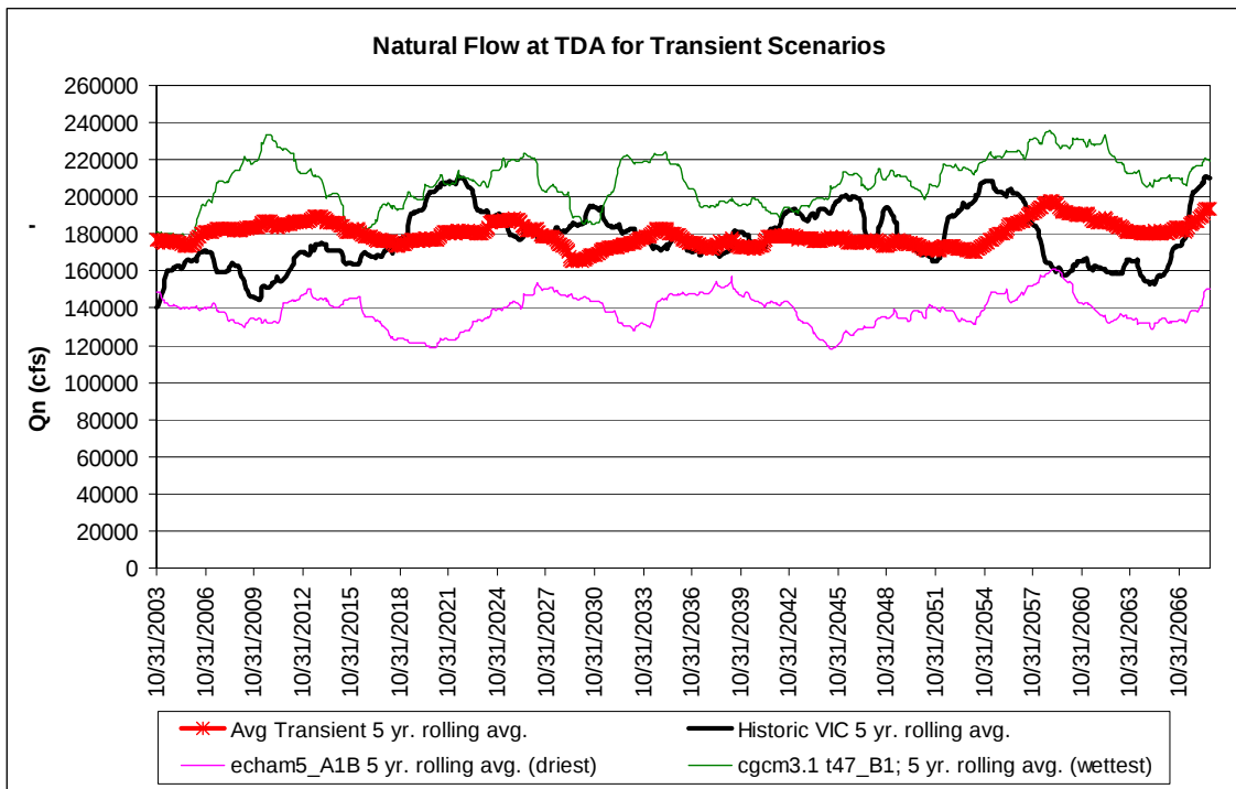
Figure 18. Natural Flows at The Dalles; 5-Yr. Rolling Average for Transient Flows.
