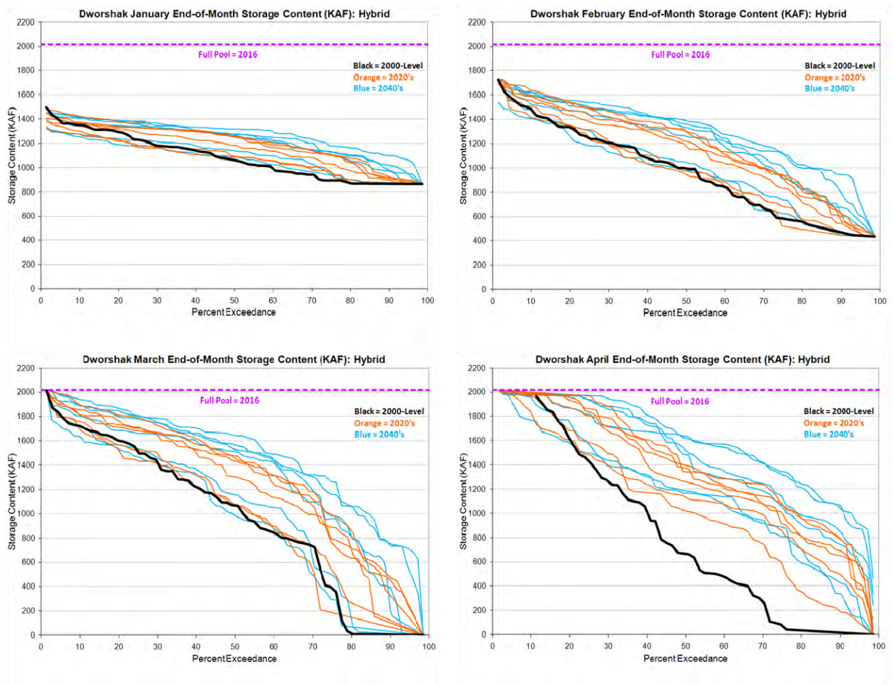
Figure 63. Dworshak Flood Control Storage Exceedance – Hybrid-Delta.
