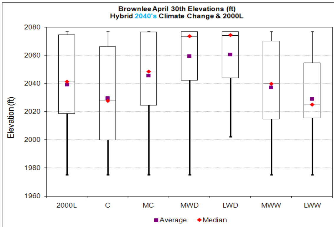
Figure 44. Brownlee April 30th Elevations, 2000 Level & Climate Change Scenarios – HD 2040s.
