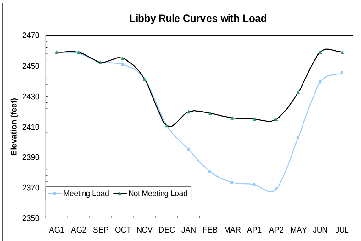
Figure 71. Libby Operating Rule Curve for FELCC Loads
