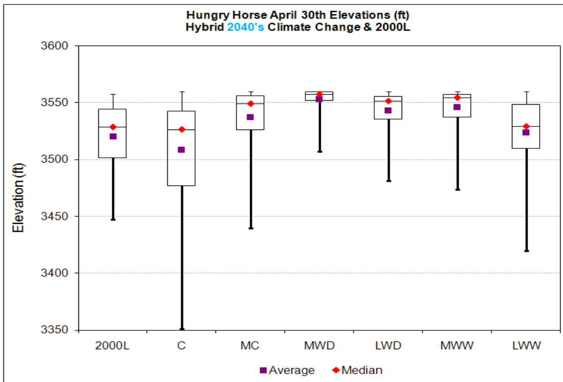
Figure 58. Hungry Horse April 30th Elevations, 2000 Level & Climate Change Scenarios – HD 2040s.
