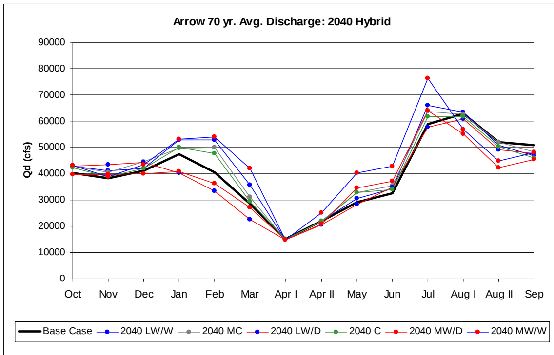
Figure 76. Arrow Discharge: 2040 Hybrid-Delta.
