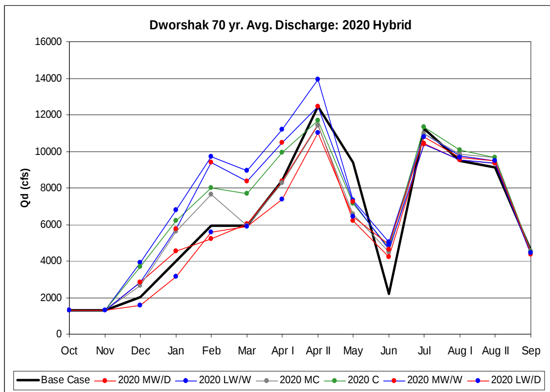
Figure 108. Dworshak seventy-year averaged Discharge: 2020s Hybrid-Delta.
