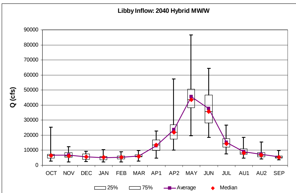
Figure 90. Libby 70 year natural inflow distribution for 2040 Hybrid-Delta MW/W study.
