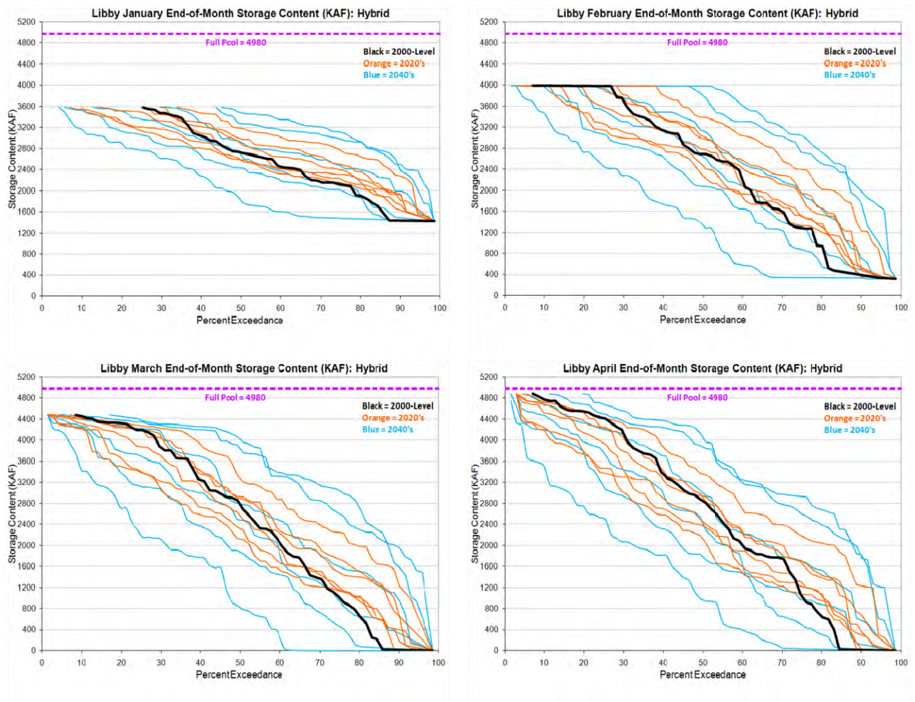
Figure 49. Libby Flood Control Storage Exceedance – Hybrid-Delta.
