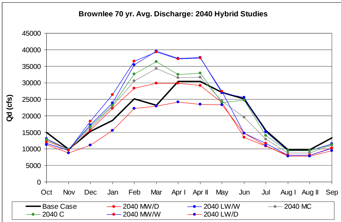
Figure 118. Brownlee monthly average discharge for each 2040 Hybrid-Delta climate change scenario.
