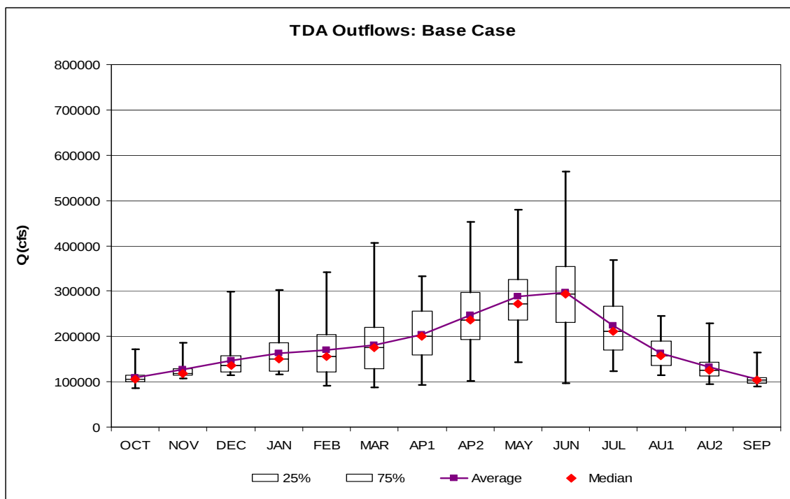
Figure 129. The Dalles Outflows for Base Case.
