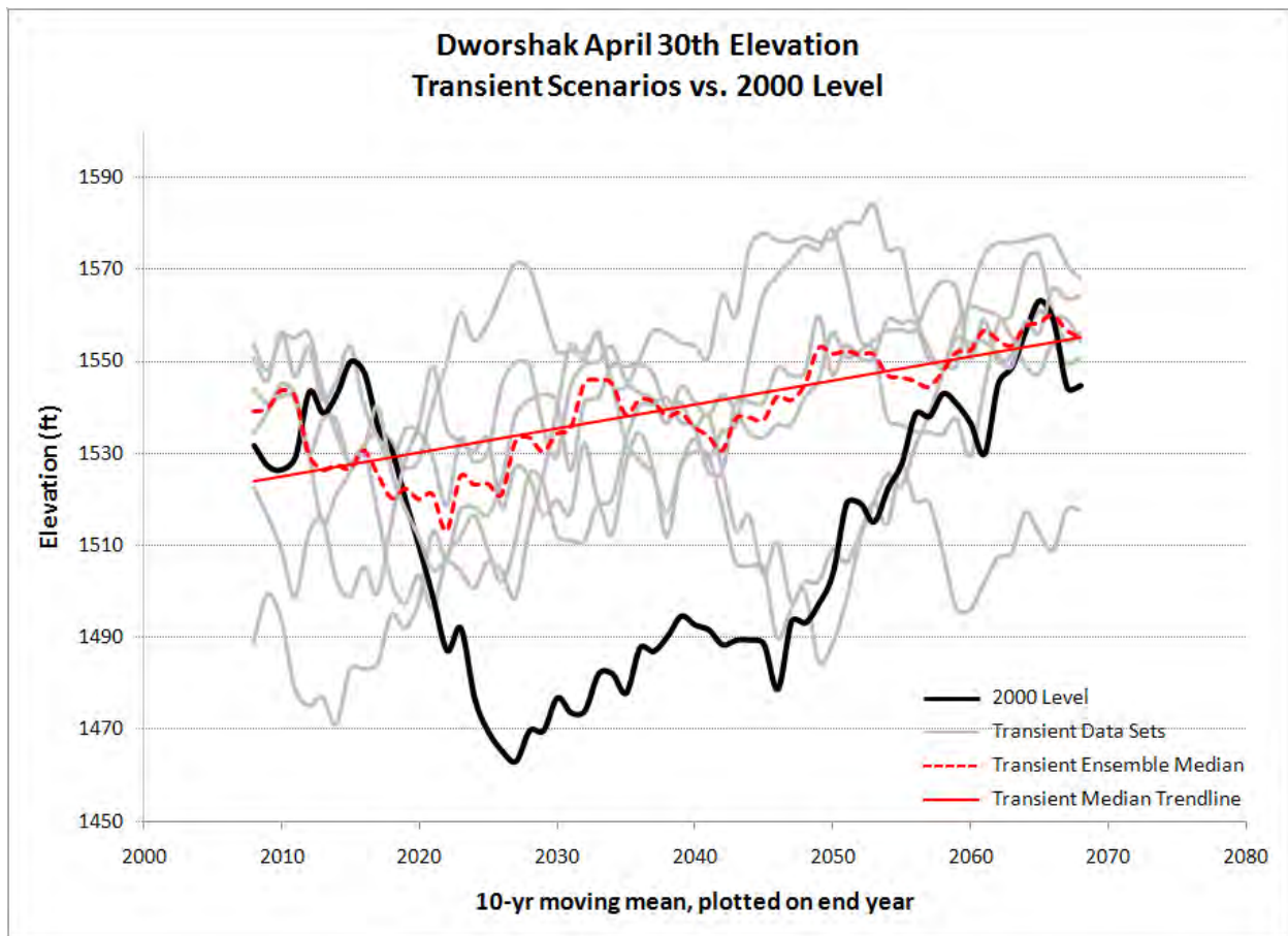
Figure 66. Dworshak 30 Elevations Rolling Average – Transient.
