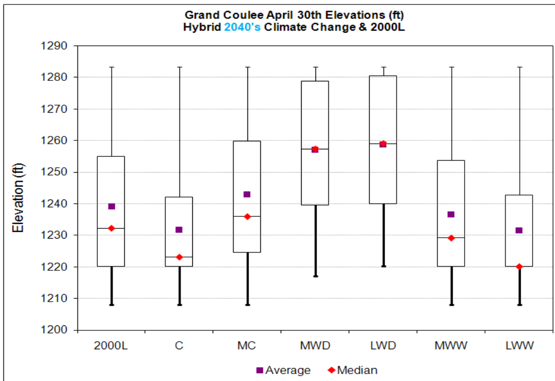
Figure 37. Grand Coulee April 30th Elevations, 2000 Level & Climate Change Scenarios–HD 2040s.
