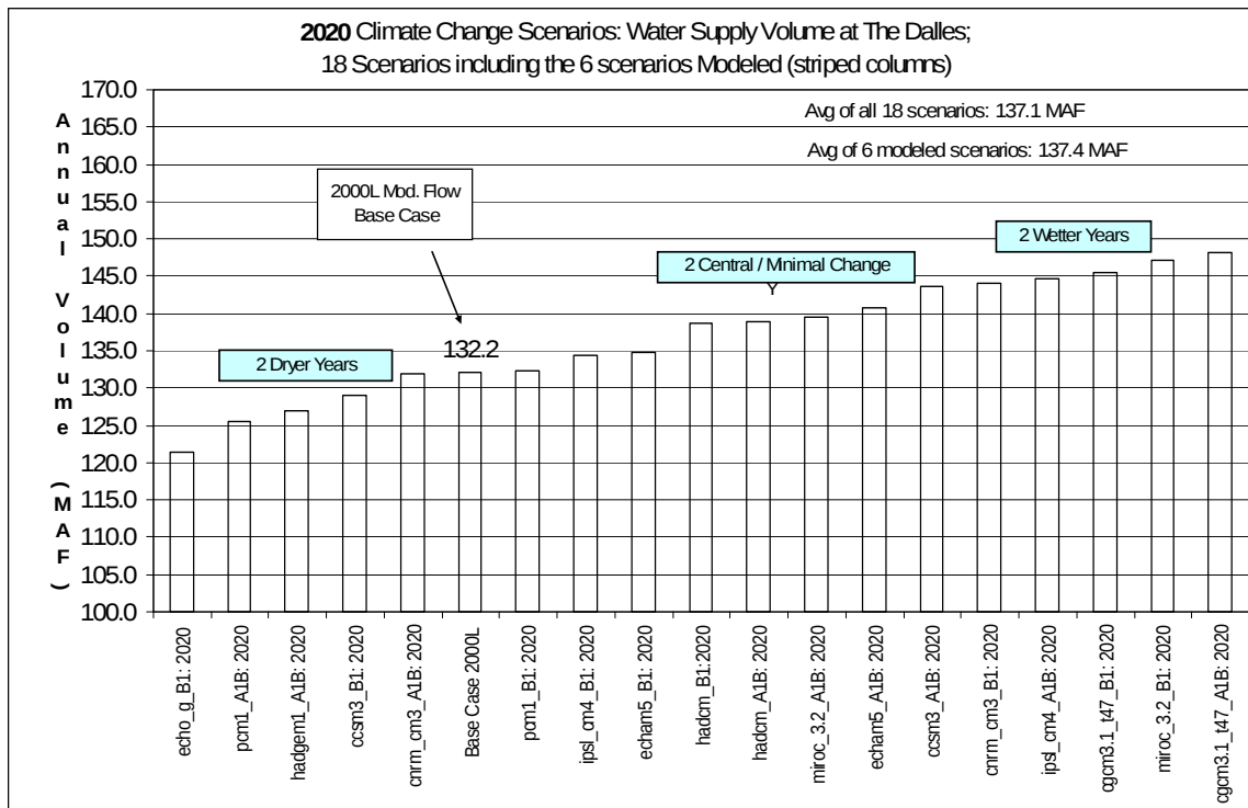
Figure 8. Annual Flow Volumes (averaged over 1929 – 1998) at TDA for 2000L Modified Flow and all 2020 Climate-Change Scenarios.
