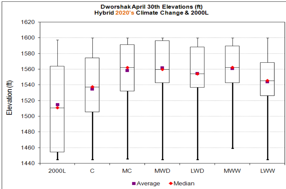
Figure 64. Dworshak April 30 Elevations, 2000 Level & Climate Change Scenarios – HD 2020s.
