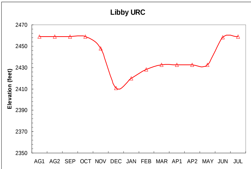
Figure 69. Libby URC for the 1937 water-year historic stream flow.
