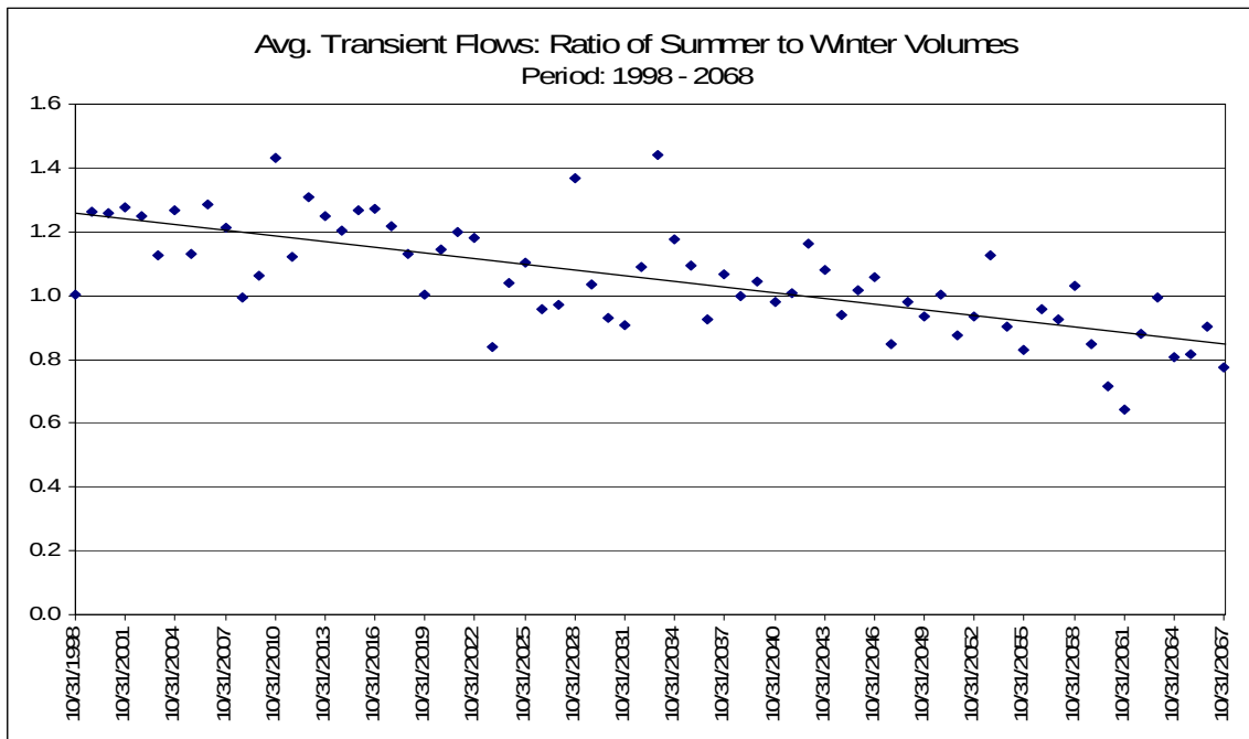
Figure 20. S/W Ratios for Transient Scenarios for the period 1999-2068.
