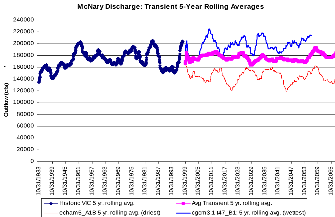
Figure 128. McNary 5-Yr. Rolling Average Discharge for Historic and Transient Scenarios.
