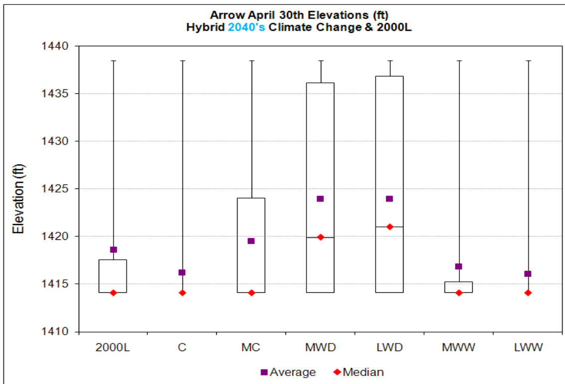
Figure 33. Arrow April 30th Elevations, 2000 Level & Climate Change Scenarios – Hybrid-Delta 2040s.
