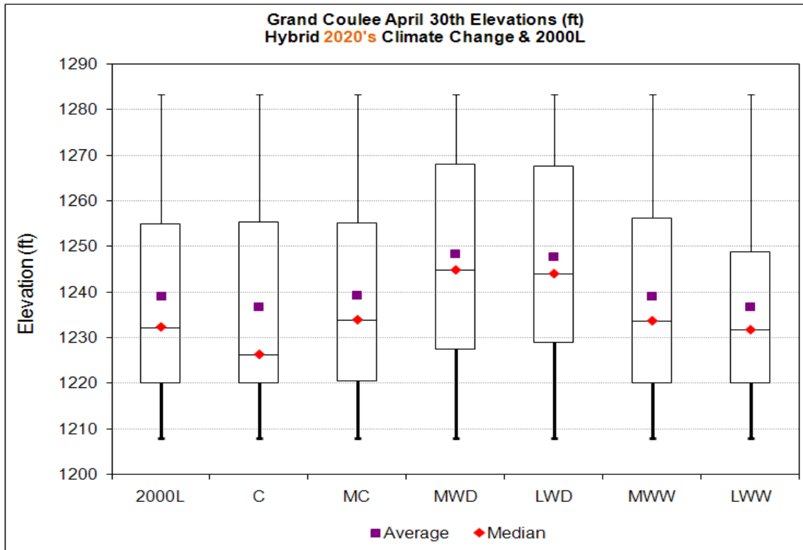
Figure 36. Grand Coulee April 30 Elevations, 2000 Level & Climate Change Scenarios–HD 2020s.
