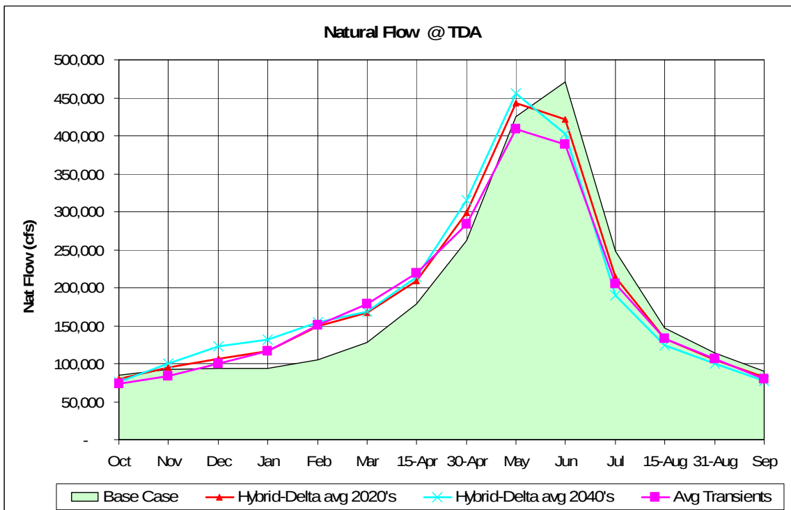
Figure 12. Natural Flows at The Dalles; Climate Change Scenario Averages.
