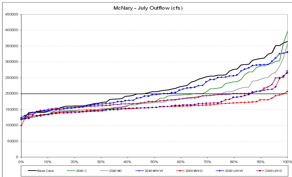
Figure 134. Comparison of 2040 Hybrid-Delta scenarios - July McNary Outflow distributions.
