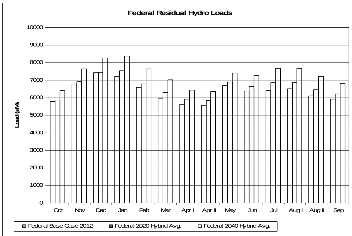
Figure 73. Federal Residual Hydro Loads.
