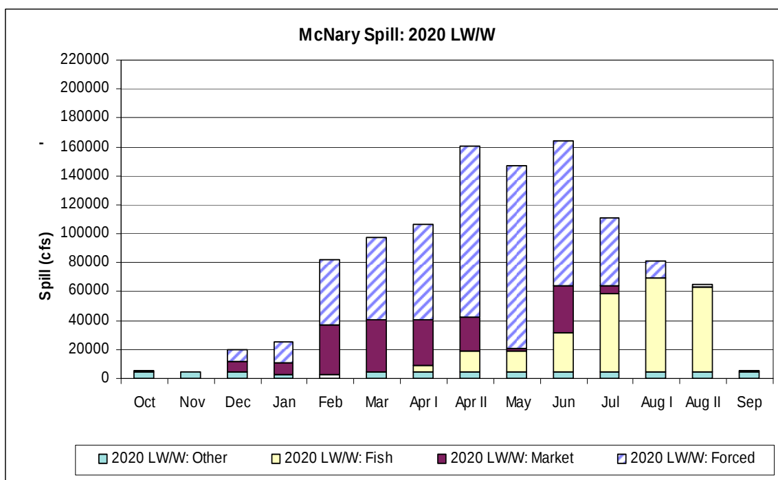
Figure 156. 2020 LW/W Scenario: McNary Spill Breakdown.
