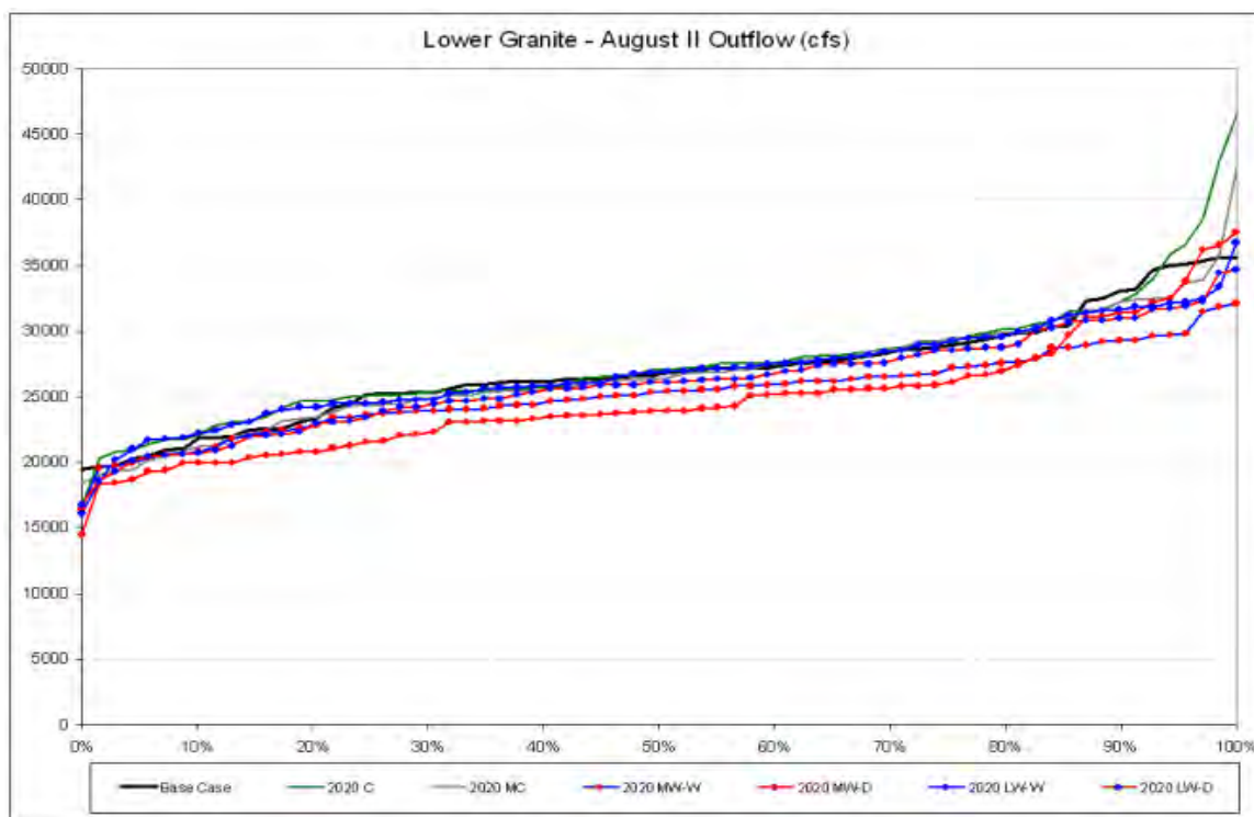
Figure 139. Comparison of 2020 Hybrid-Delta scenarios - August II Lower Granite outflow distributions.
