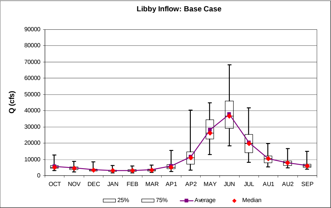
Figure 88. Libby Base Case 70 year natural inflow distribution.
