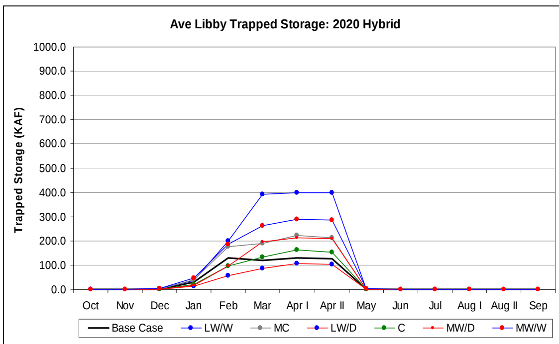
Figure 85. Average Storage trapped in Libby above required flood control due to channel restriction at Kootenay Lake in the 2020 Hybrid-Delta scenarios.
