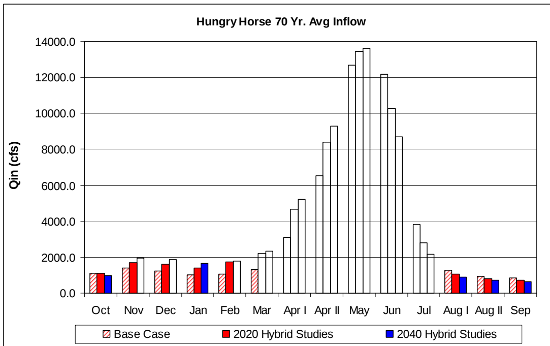
Figure 91. Hungry Horse Avg. Mo. Inflow for Base Case and Climate Change Scenarios.
