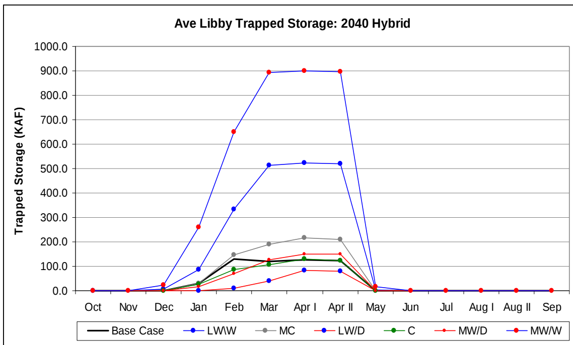
Figure 86. Average Storage trapped in Libby above required flood control due to channel restriction at Kootenay Lake in the 2040 Hybrid-Delta scenarios.
