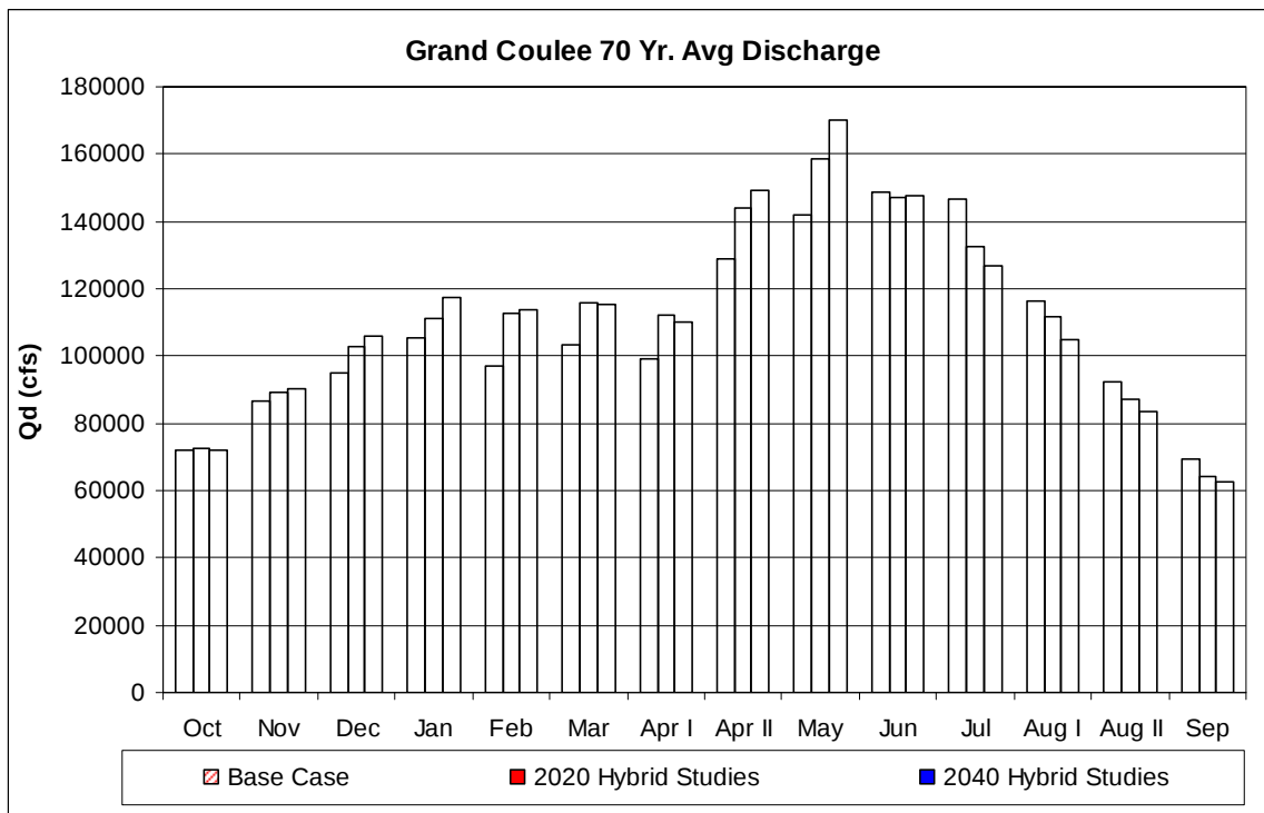
Figure 98. Grand Coulee Average Monthly Discharge for Base Case and Climate Change Scenarios.
