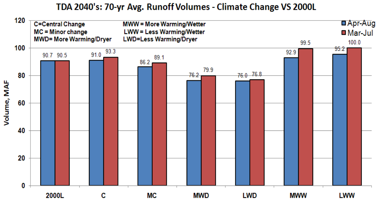
Figure 26. The Dalles Apr-Aug VS Mar-Jul Runoff Volume – Hybrid-Delta 2040s.
