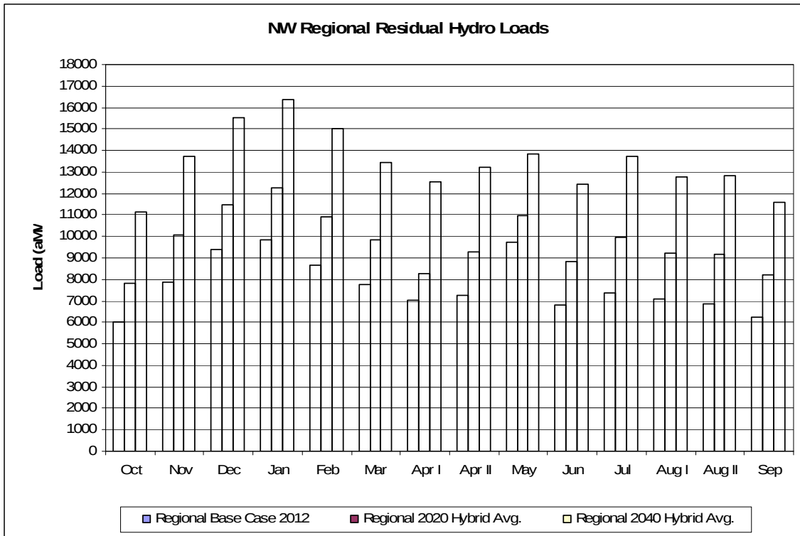
Figure 74. Regional Residual Hydro Loads.
