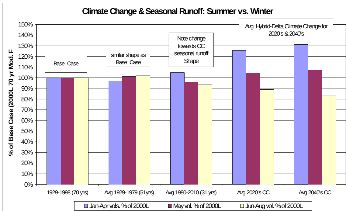
Figure 15. Summer / Winter Volumes for Historical and Future Hybrid-Delta 2020s & 2040s Scenarios.
