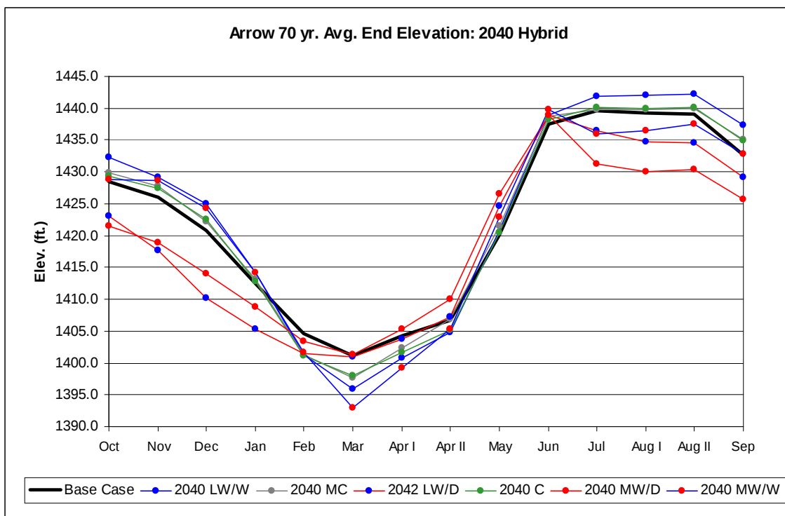
Figure 78. Arrow End Elevation: 2040s Hybrid-Delta.
