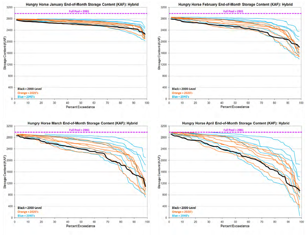
Figure 56. Hungry Horse Flood Control Storage Exceedance – Hybrid-Delta.
