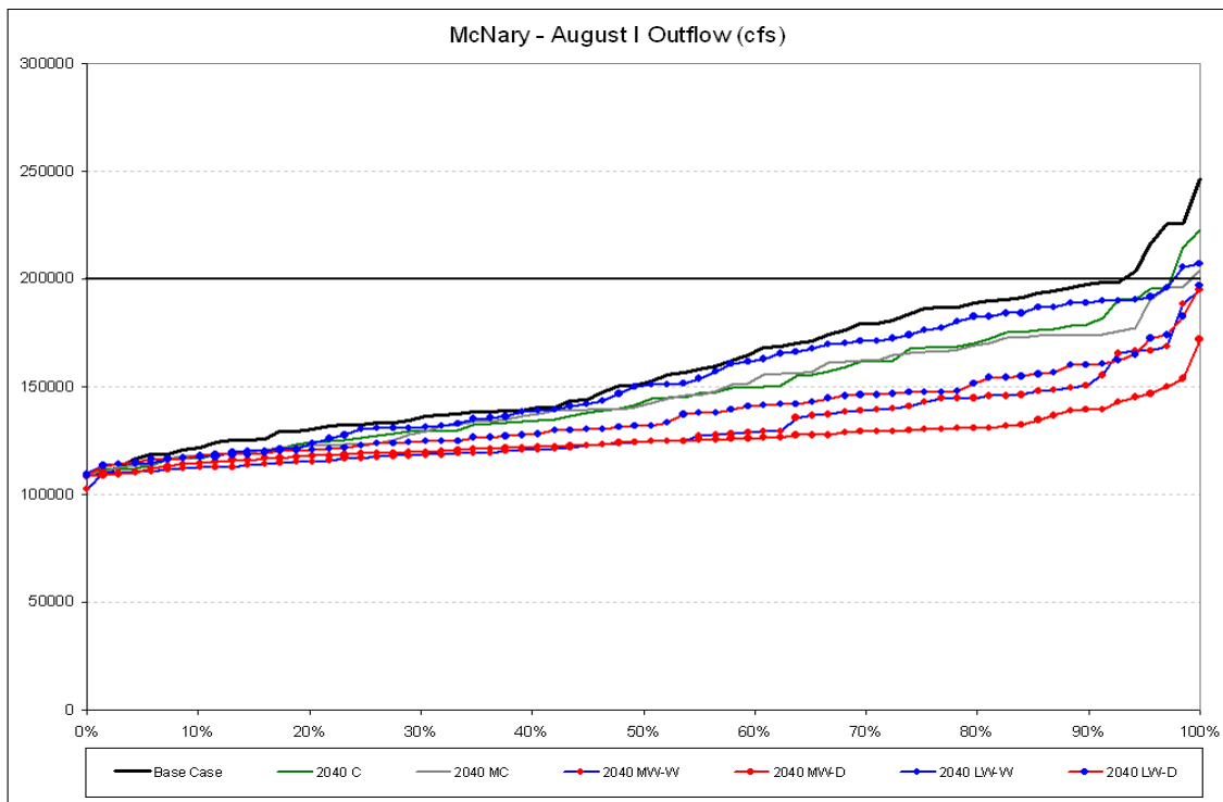
Figure 135. Comparison of 2040 Hybrid-Delta scenarios - August I McNary Outflow distributions.
