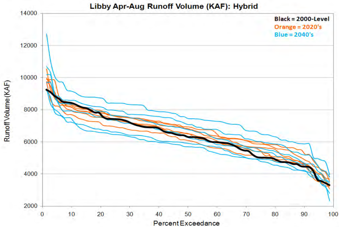
Figure 47. Libby Apr-Aug Runoff Volume Exceedance – Hybrid-Delta.
