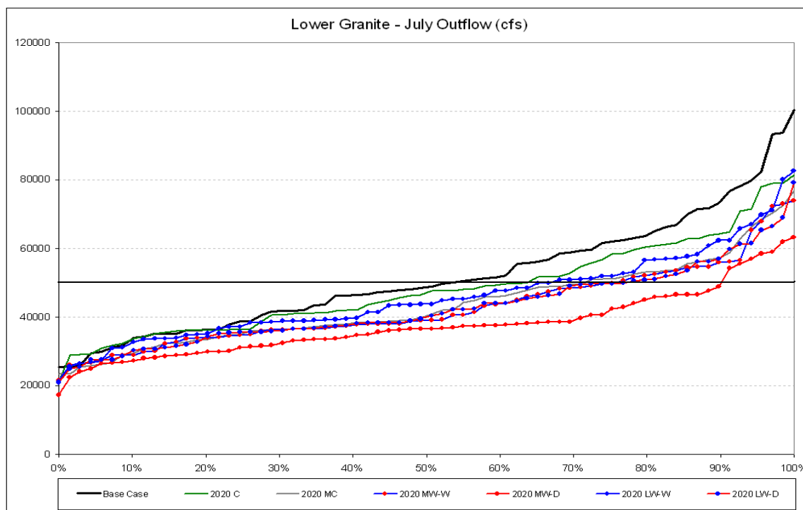
Figure 137. Comparison of 2020 Hybrid-Delta scenarios - July Lower Granite outflow distributions.
