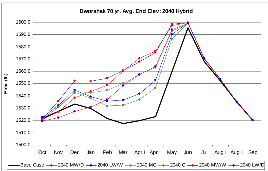
Figure 111. Dworshak End Elevations: 2040s HD.
