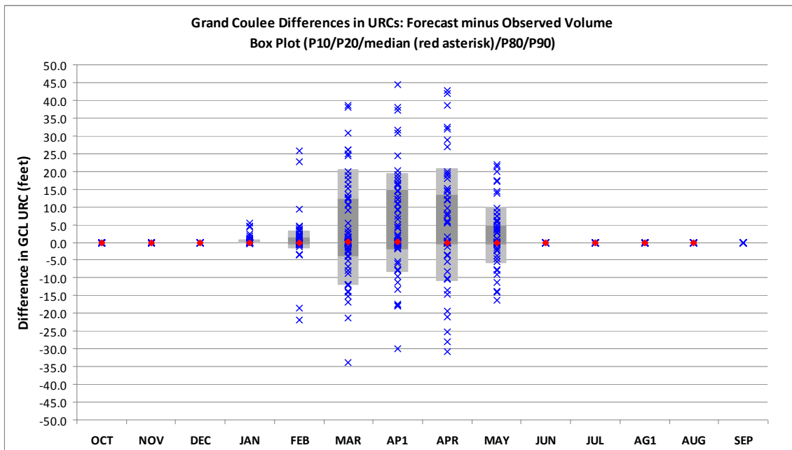
Figure 17. Grand Coulee URC Differences: Forecasted minus Observed Volumes for each of 70 years
