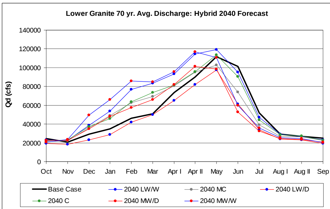
Figure 122. Lower Granite Discharge: 2040s Hybrid-Delta.
