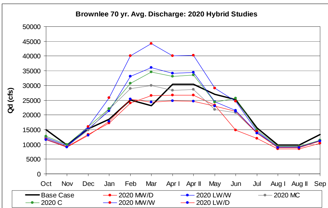
Figure 116. Brownlee month average discharge for each 2020 Hybrid-Delta climate change scenario.
