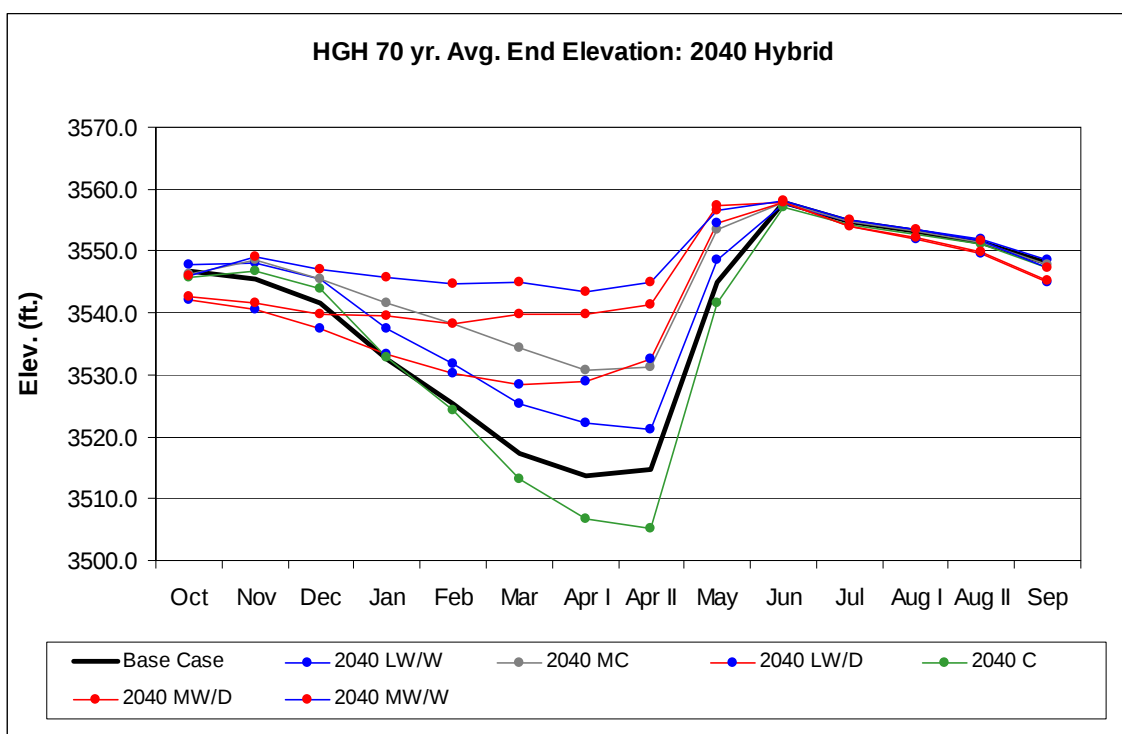
Figure 97. Hungry Horse End Elevations: 2040s HD.
