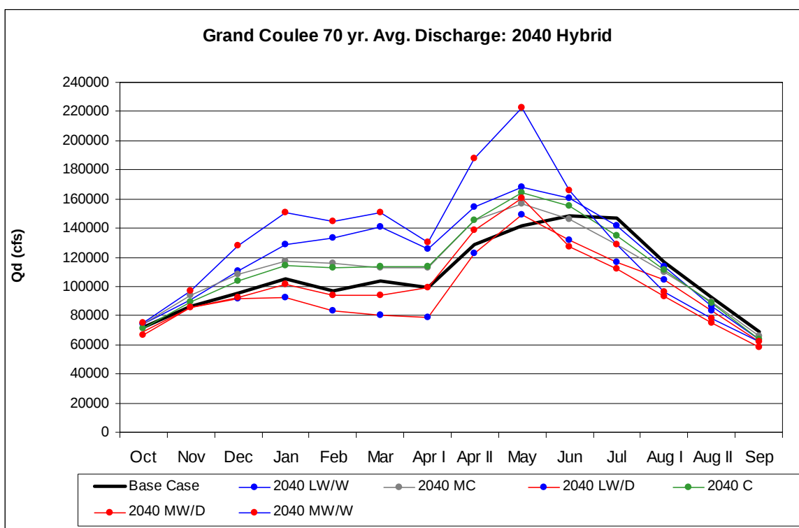
Figure 101. Grand Coulee Discharge: 2040s Hybrid-Delta.
