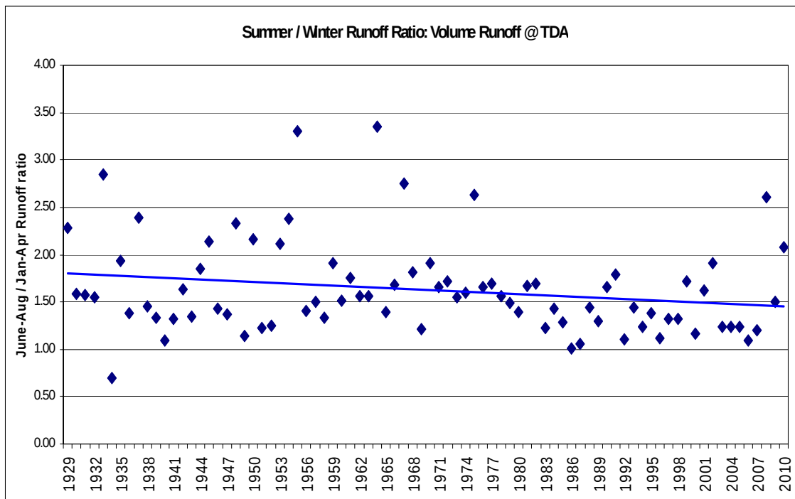
Figure 19. S/W Ratio of Runoff at TDA for the Historical period 1929-2010.
