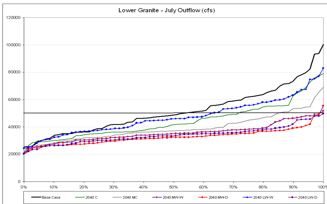
Figure 140. Comparison of 2040 Hybrid-Delta scenarios - July Lower Granite outflow distributions
