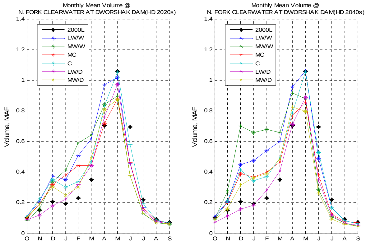
Figure 60. Dworshak Mean Monthly Volume – Hybrid-Delta.
