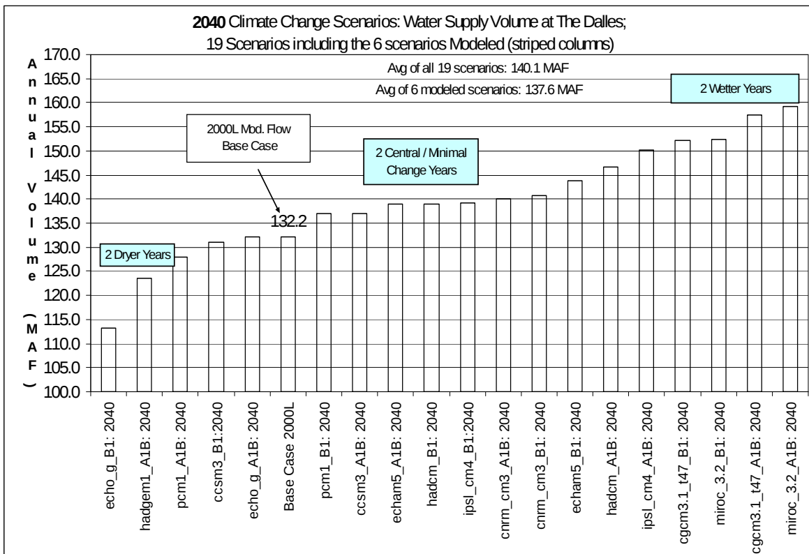
Figure 9. Annual Flow Volumes (averaged over 1929 – 1998) at TDA for 2000L Modified Flow and all 2040 Climate-Change Scenarios.
