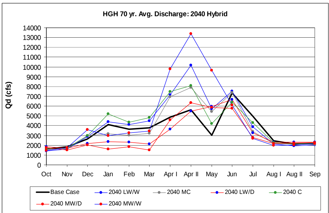
Figure 96. Hungry Horse Discharge: 2040s Hybrid-Delta.
