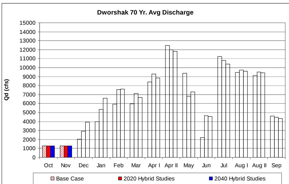
Figure 105. Dworshak Average Monthly Discharge for Base Case and Climate Change Scenarios.
